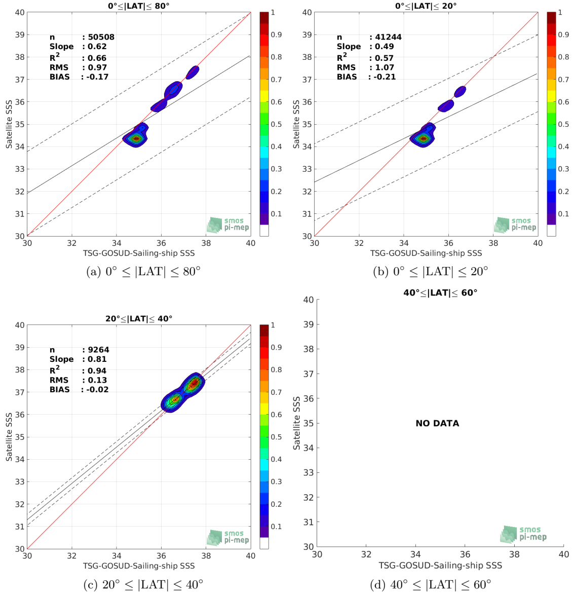
Figure 9: Contour maps of the concentration of Aquarius-L4-IPRC-V5-MONTHLY SSS (y-axis) versus TSG-GOSUD-Sailing-ship SSS (x-axis) at match-up pairs for different latitude bands. For each plot, the red line shows x=y . The black thin and dashed lines indicate a linear fit through the data cloud and the \pm 95\% confidence levels, respectively. The number match-up pairs n , the slope and R^2 coefficient of the linear fit, the root mean square (RMS) and the mean bias between satellite and in situ data are indicated for each latitude band in each plots.
