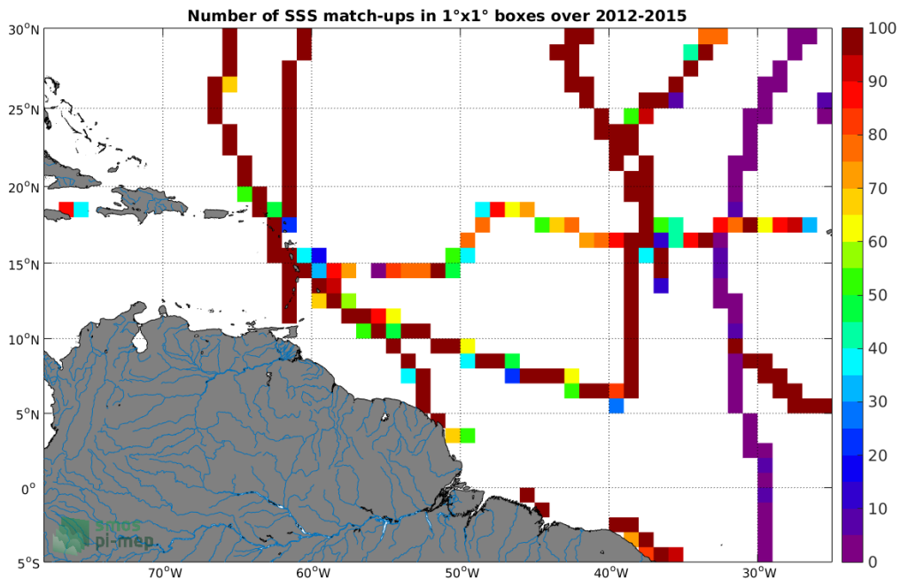
Figure 4: Number of SSS match-ups between TSG-GOSUD-Sailing-ship SSS and the Aquarius-L4-IPRC-V5-MONTHLY SSS product for the Amazon and Orinoco river plumes Pi-MEP region over 1°x1° boxes and for the full satellite product period.
