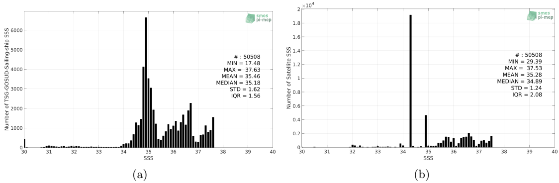
Figure 2: Histograms of SSS from TSG-GOSUD-Sailing-ship (a) and Aquarius-L4-IPRC-V5-MONTHLY (b) considering all match-up pairs per bins of 0.1 over the Amazon and Orinoco river plumes Pi-MEP region and for the full satellite product period.
