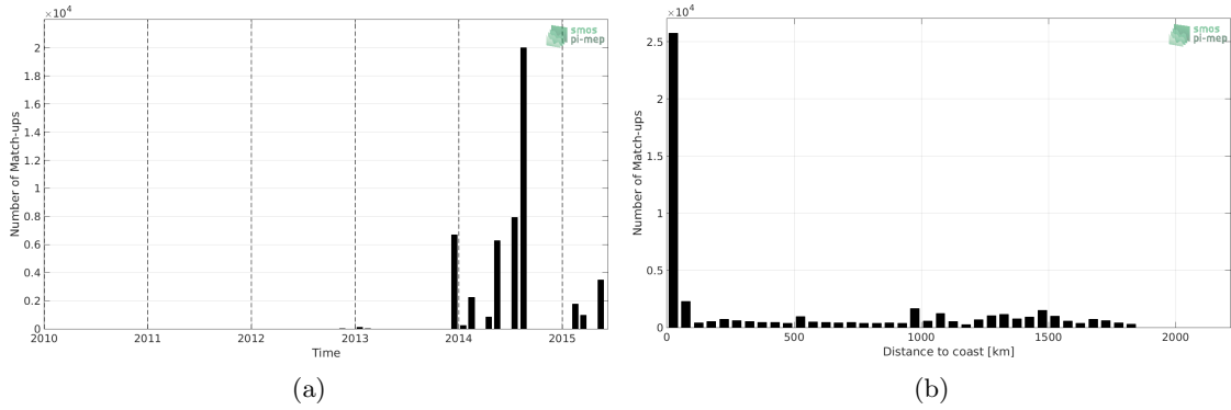
Figure 1: Number of match-ups between TSG-GOSUD-Sailing-ship and Aquarius-L4-IPRC-V5-MONTHLY SSS as a function of time (a) and as function of the distance to coast (b) over the Amazon and Orinoco river plumes Pi-MEP region and for the full satellite product period.
