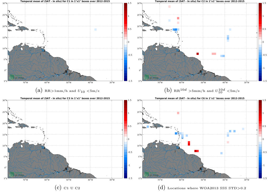
Figure 12: Temporal mean gridded over spatial boxes of size 1^\circ \times 1^\circ of \Delta SSS (Aquarius-L4-IPRC-V5-MONTHLY - TSG-GOSUD-Sailing-ship) for 4 different subdatasets corresponding to: RR > 1\text{mm/h} and U_{10} < 5\text{m/s} (a), RR^{10d} > 5\text{mm/h} and U_{10}^{10d} < 5\text{m/s} (b), C1 U C2 (c), Locations where WOA2013 SSS STD > 0.2 (d).
