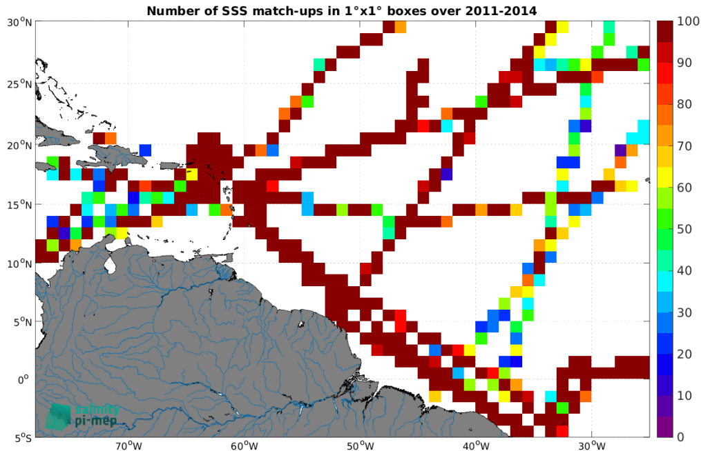
Figure 5: Number of SSS match-ups between TSG (GOSUD-Research-vessel) SSS and the Aquarius SSS L4 OI v5 - Monthly (IPRC) SSS product for the Amazon and Orinoco river plumes Pi-MEP region over 1^\circ \times 1^\circ boxes and for the full satellite product period.
