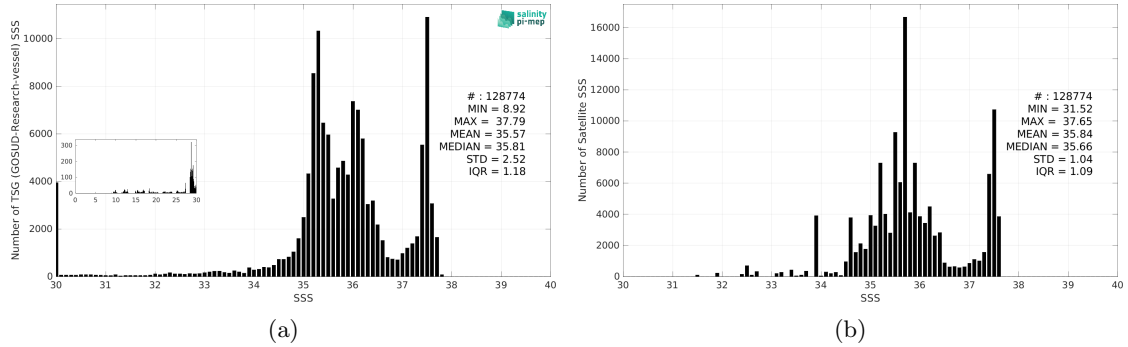
Figure 3: Histograms of SSS from TSG (GOSUD-Research-vessel) (a) and Aquarius SSS L4 OI v5 - Monthly (IPRC) (b) considering all match-up pairs per bins of 0.1 over the Amazon and Orinoco river plumes Pi-MEP region and for the full satellite product period.
