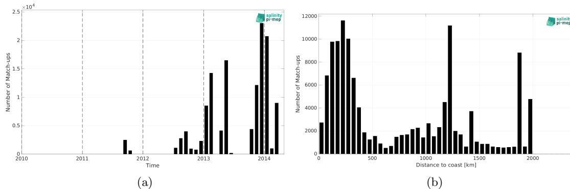
Figure 2: Number of match-ups between TSG (GOSUD-Research-vessel) and Aquarius SSS L4 OI v5 - Monthly (IPRC) SSS as a function of time (a) and as function of the distance to coast (b) over the Amazon and Orinoco river plumes Pi-MEP region and for the full satellite product period.
