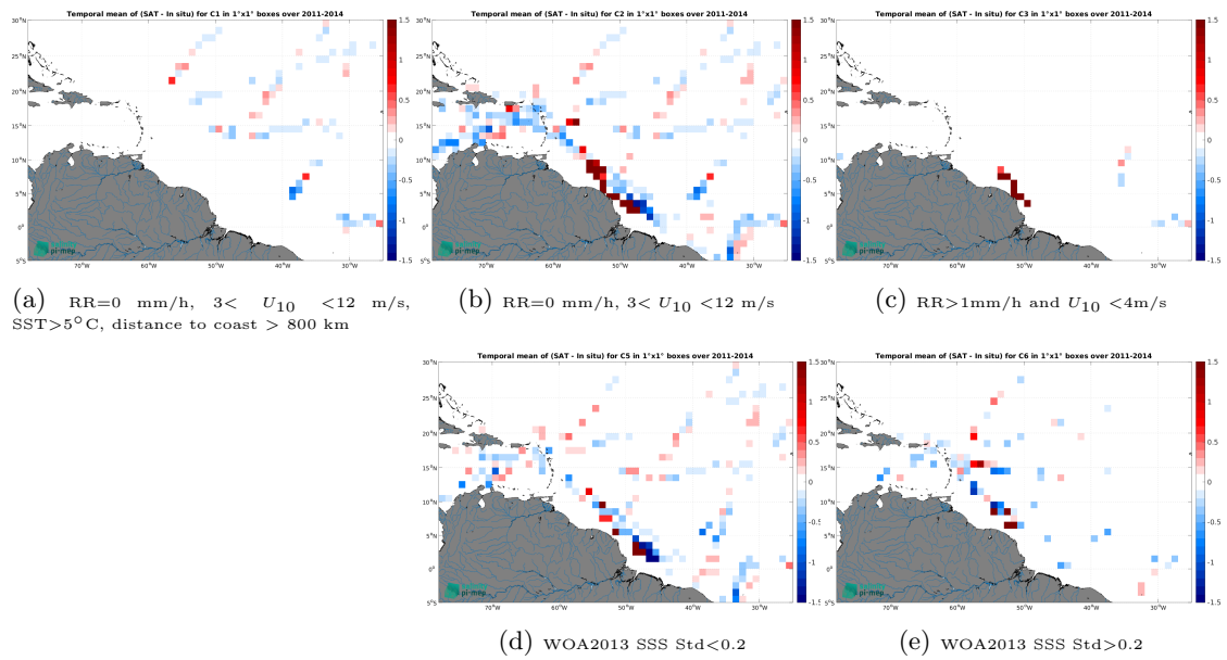
Figure 12: Temporal mean gridded over spatial boxes of size 1^\circ \times 1^\circ of \Delta\text{SSS} (Aquarius SSS L4 OI v5 - Monthly (IPRC) - TSG (GOSUD-Research-vessel)) for 5 different subdatasets corresponding to:RR=0 mm/h, 3 < U_{10} < 12 m/s, SST>5°C, distance to coast > 800 km (a), RR=0 mm/h, 3 < U_{10} < 12 m/s (b), RR>1mm/h and U_{10} < 4 m/s (c), WOA2013 SSS Std<0.2 (d), WOA2013 SSS Std>0.2 (e).
