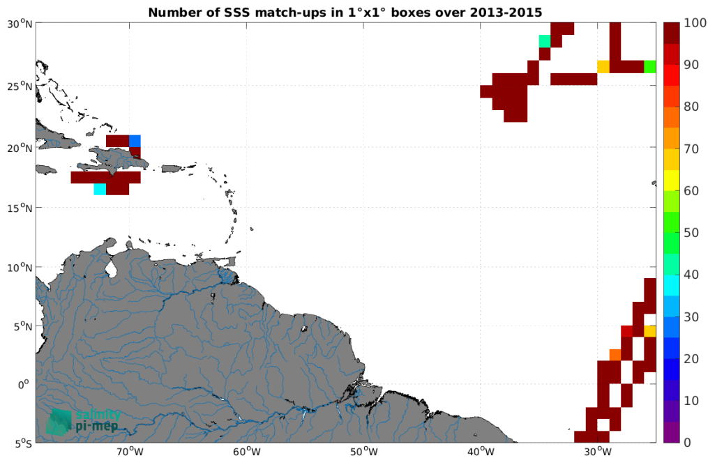
Figure 5: Number of SSS match-ups between TSG (CSIC-UTM) SSS and the Aquarius SSS L4 OI v5 - Monthly (IPRC) SSS product for the Amazon and Orinoco river plumes Pi-MEP region over 1^\circ \times 1^\circ boxes and for the full satellite product period.
