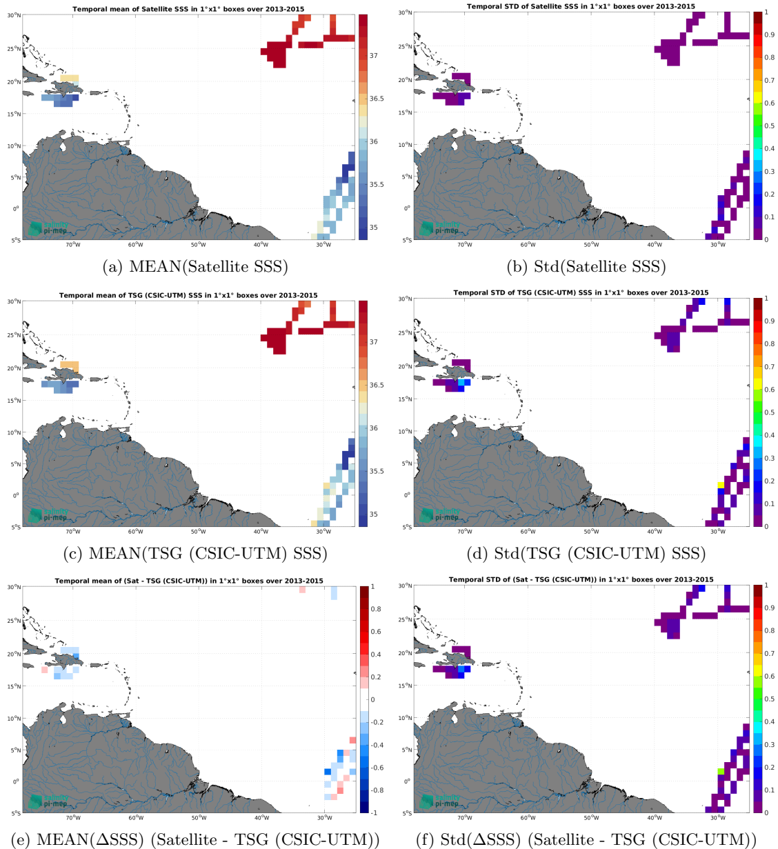
Figure 7: Temporal mean (left) and Std (right) of SSS from Aquarius SSS L4 OI v5 - Monthly (IPRC) (top), TSG (CSIC-UTM) (middle), and of \Delta SSS (Satellite - TSG (CSIC-UTM)). Only match-up pairs are used to generate these maps.
