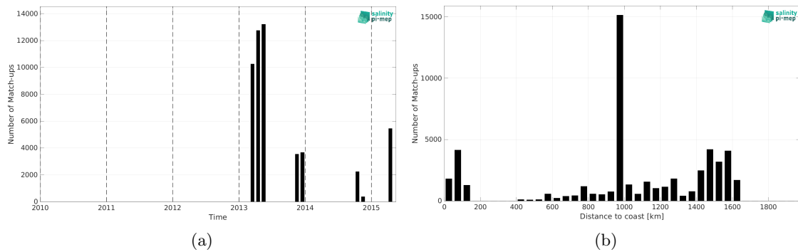
Figure 2: Number of match-ups between TSG (CSIC-UTM) and Aquarius SSS L4 OI v5 - Monthly (IPRC) SSS as a function of time (a) and as function of the distance to coast (b) over the Amazon and Orinoco river plumes Pi-MEP region and for the full satellite product period.
