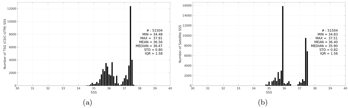
Figure 3: Histograms of SSS from TSG (CSIC-UTM) (a) and Aquarius SSS L4 OI v5 - Monthly (IPRC) (b) considering all match-up pairs per bins of 0.1 over the Amazon and Orinoco river plumes Pi-MEP region and for the full satellite product period.
