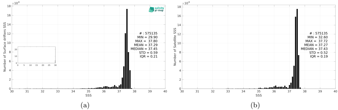
Figure 3: Histograms of SSS from Surface drifters (a) and Aquarius SSS L4 OI v5 - Monthly (IPRC) (b) considering all match-up pairs per bins of 0.1 over the Amazon and Orinoco river plumes Pi-MEP region and for the full satellite product period.
