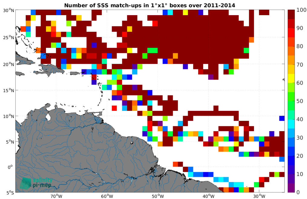
Figure 4: Number of SSS match-ups between Surface drifters SSS and the Aquarius SSS L4 OI v5 - Monthly (IPRC) SSS product for the Amazon and Orinoco river plumes Pi-MEP region over 1^\circ \times 1^\circ boxes and for the full satellite product period.
