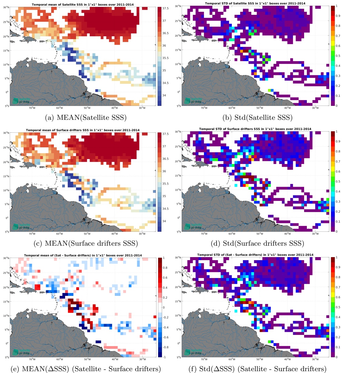
Figure 6: Temporal mean (left) and Std (right) of SSS from Aquarius SSS L4 OI v5 - Monthly (IPRC) (top), Surface drifters (middle), and of \Delta SSS (Satellite - Surface drifters). Only match-up pairs are used to generate these maps.
