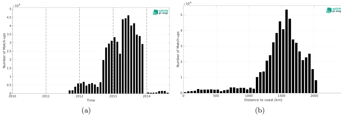
Figure 2: Number of match-ups between Surface drifters and Aquarius SSS L4 OI v5 - Monthly (IPRC) SSS as a function of time (a) and as function of the distance to coast (b) over the Amazon and Orinoco river plumes Pi-MEP region and for the full satellite product period.
