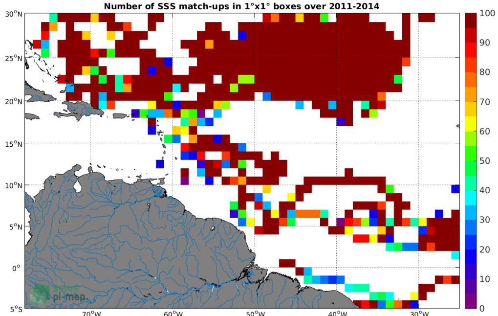
Figure 3: Number of SSS match-ups between Surface drifters SSS and the Aquarius-L4-IPRC-V5-MONTHLY SSS product for the Amazon and Orinoco river plumes Pi-MEP region over 1^\circ \times 1^\circ boxes and for the full satellite product period.
