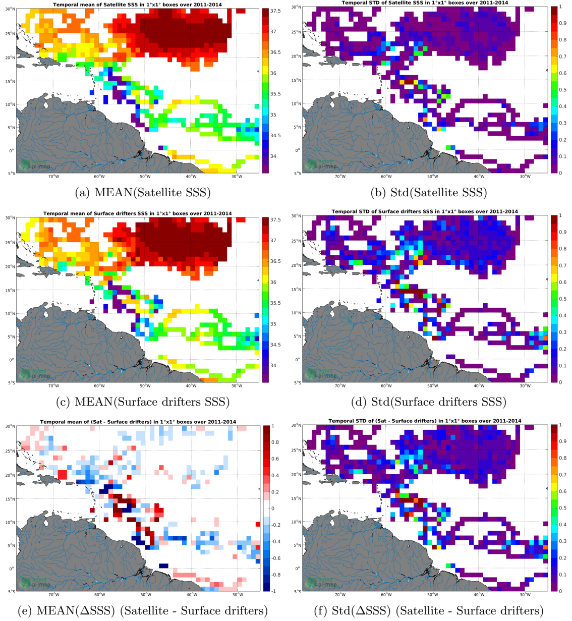
Figure 5: Temporal mean (left) and Std (right) of SSS from Aquarius-L4-IPRC-V5-MONTHLY (top), Surface drifters (middle), and of \Delta SSS (Satellite - Surface drifters). Only match-up pairs are used to generate these maps.
