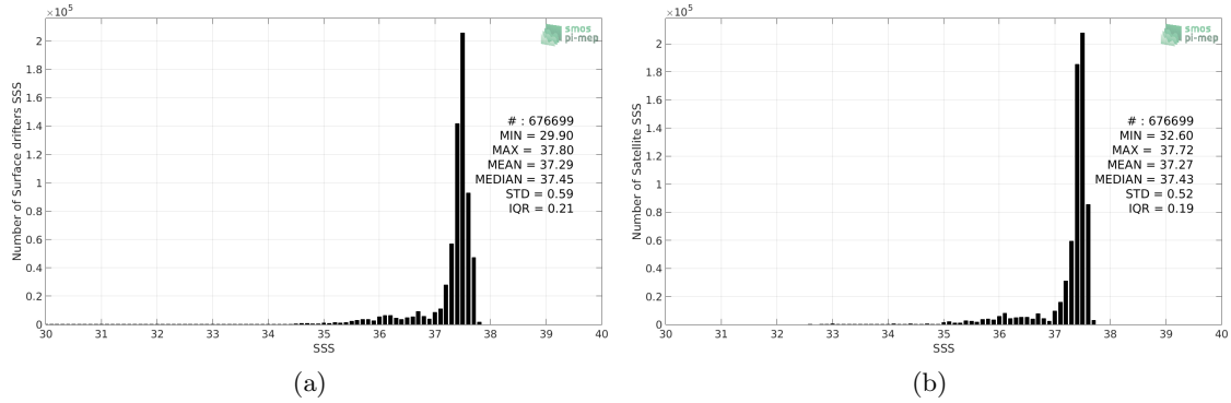
Figure 2: Histograms of SSS from Surface drifters (a) and Aquarius-L4-IPRC-V5-MONTHLY (b) considering all match-up pairs per bins of 0.1 over the Amazon and Orinoco river plumes Pi-MEP region and for the full satellite product period.
