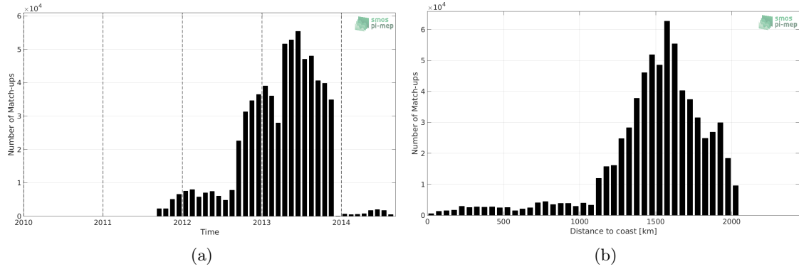
Figure 1: Number of match-ups between Surface drifters and Aquarius-L4-IPRC-V5-MONTHLY SSS as a function of time (a) and as function of the distance to coast (b) over the Amazon and Orinoco river plumes Pi-MEP region and for the full satellite product period.
