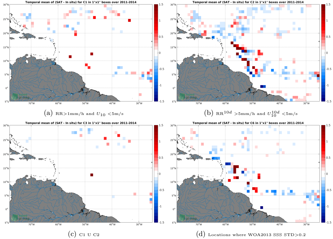
Figure 11: Temporal mean gridded over spatial boxes of size 1^\circ \times 1^\circ of \Delta SSS (Aquarius-L4-IPRC-V5-MONTHLY - Surface drifters) for 4 different subdatasets corresponding to: RR > 1\text{mm/h} and U_{10} < 5\text{m/s} (a), RR^{10d} > 5\text{mm/h} and U_{10}^{10d} < 5\text{m/s} (b), C1 U C2 (c), Locations where WOA2013 SSS STD > 0.2 (d).
