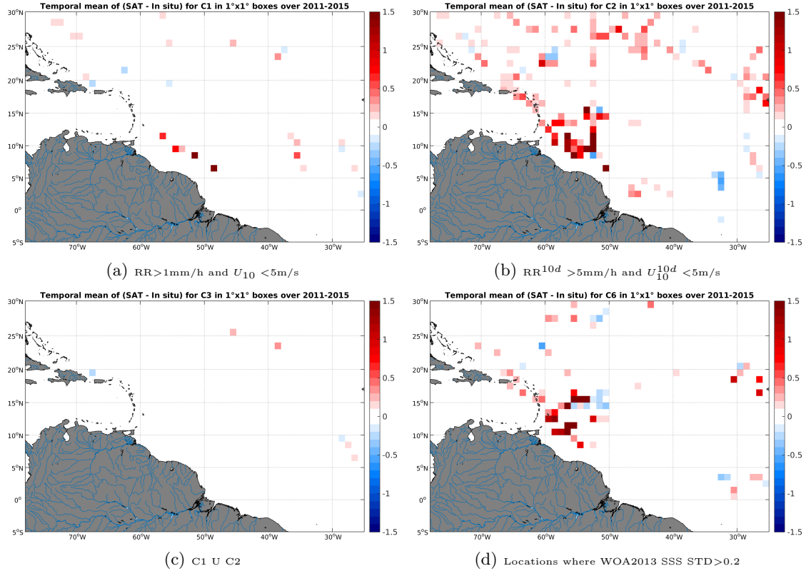
Figure 12: Temporal mean gridded over spatial boxes of size 1^\circ \times 1^\circ of \Delta SSS (Aquarius-L4-IPRC-V4-WEEKLY - TSG-SAMOS) for 4 different subdatasets corresponding to: RR > 1mm/h and U_{10} < 5 m/s (a), RR^{10d} > 5 mm/h and U_{10}^{10d} < 5 m/s (b), C1 U C2 (c), Locations where WOA2013 SSS STD > 0.2 (d).
