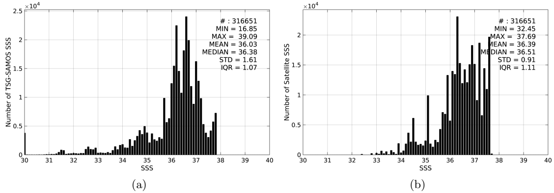
Figure 2: Histograms of SSS from TSG-SAMOS (a) and Aquarius-L4-IPRC-V4-WEEKLY (b) considering all match-up pairs per bins of 0.1 over the Amazon and Orinoco river plumes Pi-MEP region and for the full satellite product period.
