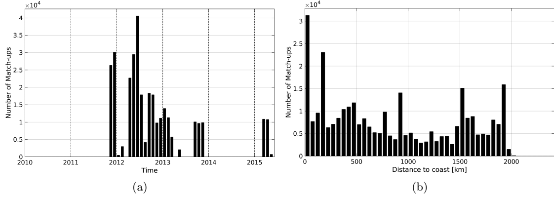
Figure 1: Number of match-ups between TSG-SAMOS and Aquarius-L4-IPRC-V4-WEEKLY SSS as a function of time (a) and as function of the distance to coast (b) over the Amazon and Orinoco river plumes Pi-MEP region and for the full satellite product period.
