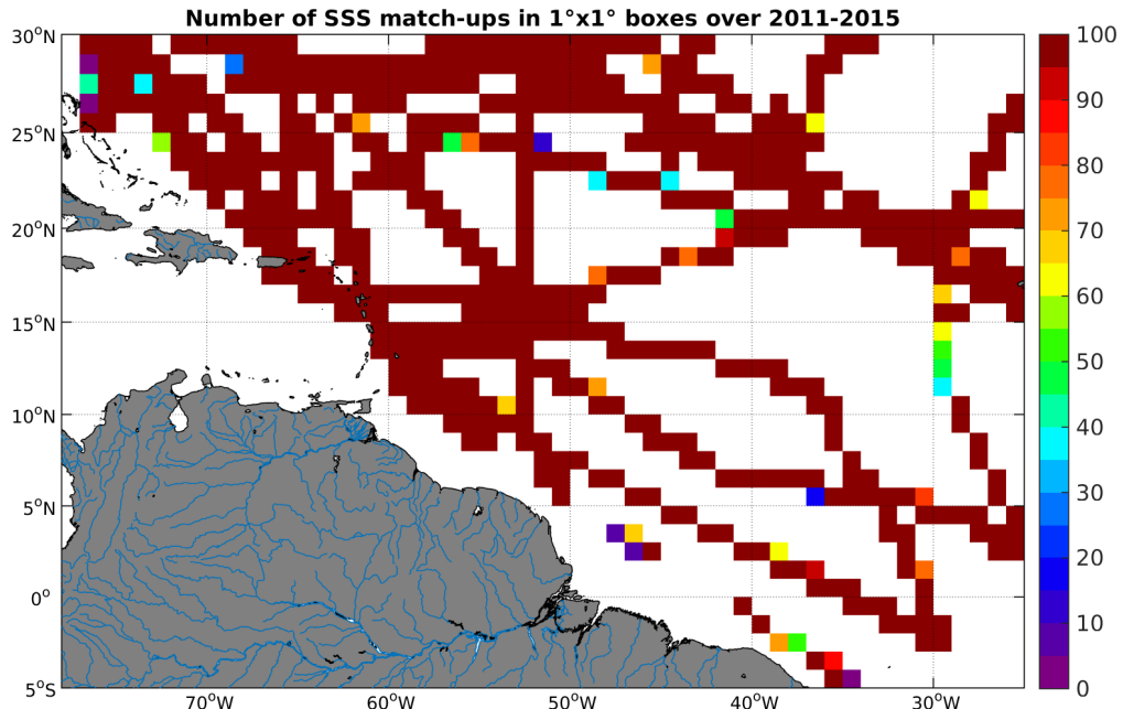
Figure 4: Number of SSS match-ups between TSG-SAMOS SSS and the Aquarius-L4-IPRC-V4-WEEKLY SSS product for the Amazon and Orinoco river plumes Pi-MEP region over 1^\circ \times 1^\circ boxes and for the full satellite product period.
