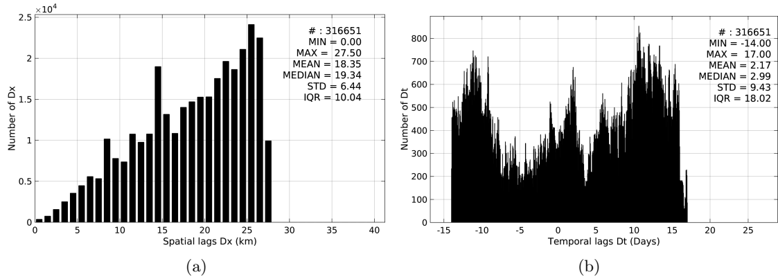
Figure 5: Histograms of the spatial (a) and temporal (b) lags between the time of the TSG-SAMOS measurements and the date of the corresponding Aquarius-L4-IPRC-V4-MONTHLY SSS product.
