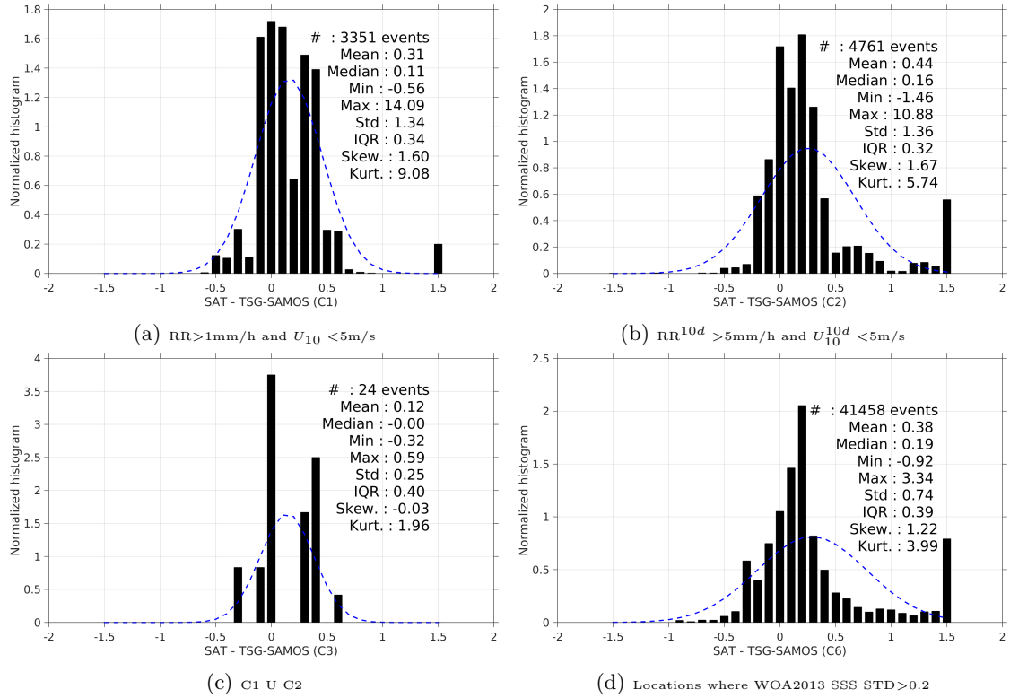
Figure 13: Normalized histogram of \Delta SSS (Aquarius-L4-IPRC-V4-MONTHLY - TSG-SAMOS) for 6 different subdatasets corresponding to: RR > 1\text{mm/h} and U_{10} < 5\text{m/s} (a), RR^{10d} > 5\text{mm/h} and U_{10}^{10d} < 5\text{m/s} (b), C1 U C2 (c), Locations where WOA2013 SSS STD > 0.2 (d).
