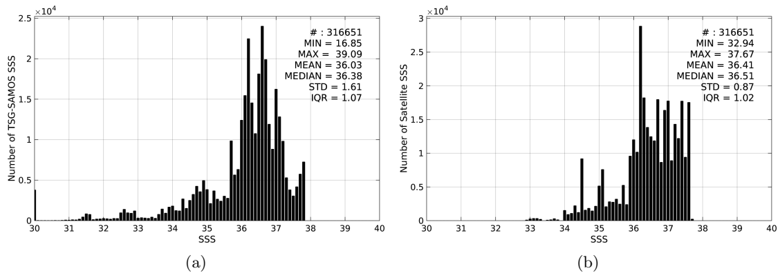
Figure 2: Histograms of SSS from TSG-SAMOS (a) and Aquarius-L4-IPRC-V4-MONTHLY (b) considering all match-up pairs per bins of 0.1 over the Amazon and Orinoco river plumes Pi-MEP region and for the full satellite product period.
