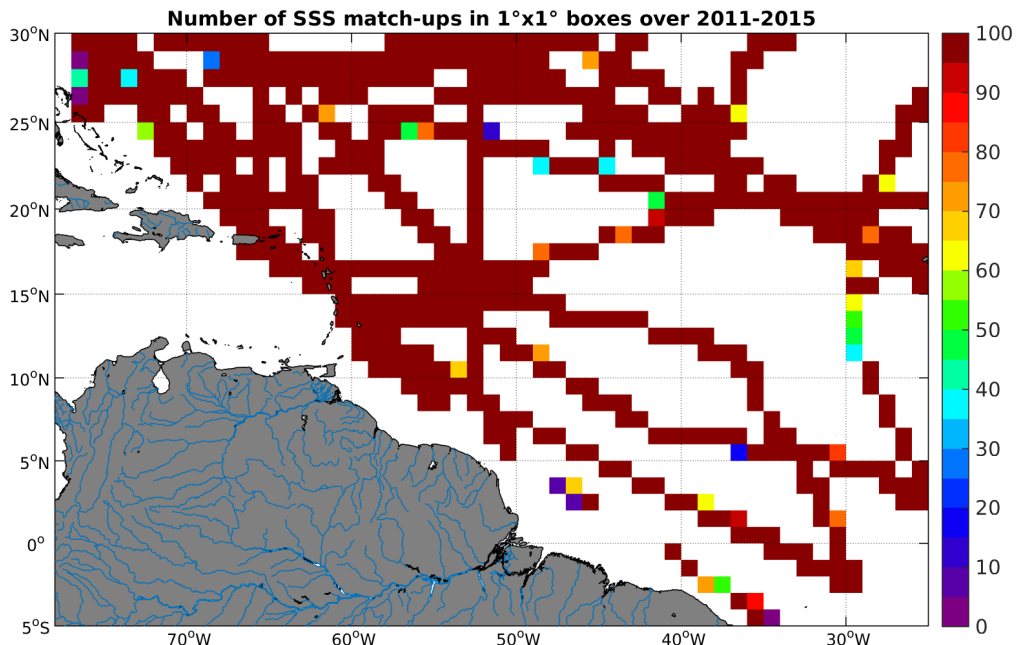
Figure 4: Number of SSS match-ups between TSG-SAMOS SSS and the Aquarius-L4-IPRC-V4-MONTHLY SSS product for the Amazon and Orinoco river plumes Pi-MEP region over 1^\circ \times 1^\circ boxes and for the full satellite product period.
