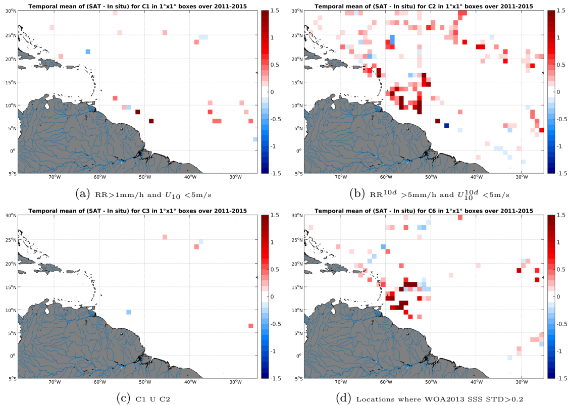
Figure 12: Temporal mean gridded over spatial boxes of size 1^\circ \times 1^\circ of \Delta SSS (Aquarius-L4-IPRC-V4-MONTHLY - TSG-SAMOS) for 4 different subdatasets corresponding to:RR >1 mm/h and U_{10} < 5 m/s (a), RR^{10d} > 5 mm/h and U_{10}^{10d} < 5 m/s (b), C1 U C2 (c),Locations where WOA2013 SSS STD >0.2 (d).
