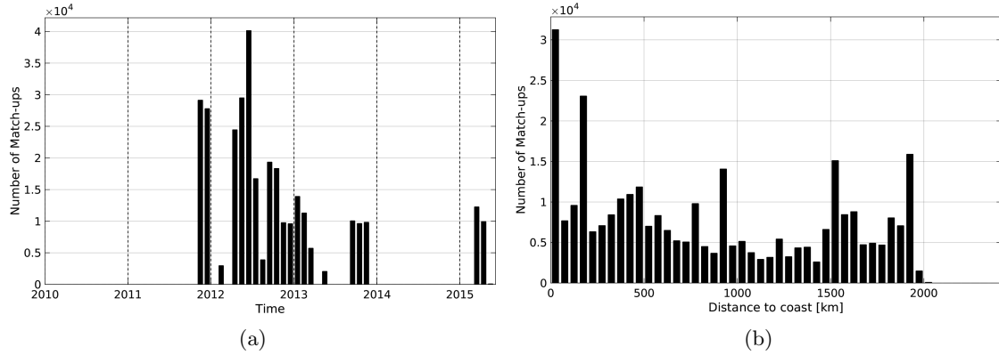
Figure 1: Number of match-ups between TSG-SAMOS and Aquarius-L4-IPRC-V4-MONTHLY SSS as a function of time (a) and as function of the distance to coast (b) over the Amazon and Orinoco river plumes Pi-MEP region and for the full satellite product period.
