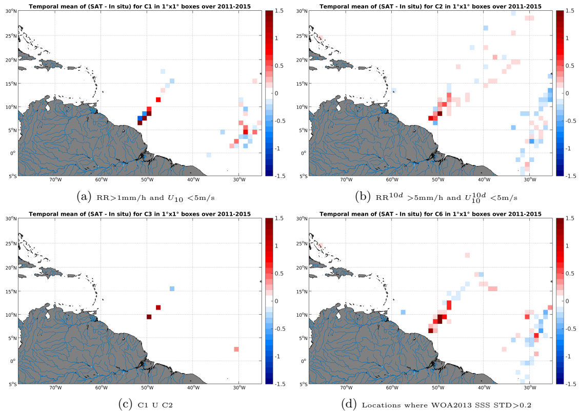
Figure 12: Temporal mean gridded over spatial boxes of size 1^\circ \times 1^\circ of \Delta SSS (Aquarius-L4-IPRC-V4-MONTHLY - TSG-LEGOS-DM) for 4 different subdatasets corresponding to: RR > 1\text{mm/h} and U_{10} < 5\text{m/s} (a), RR^{10d} > 5\text{mm/h} and U_{10}^{10d} < 5\text{m/s} (b), C1 U C2 (c), Locations where WOA2013 SSS STD > 0.2 (d).
