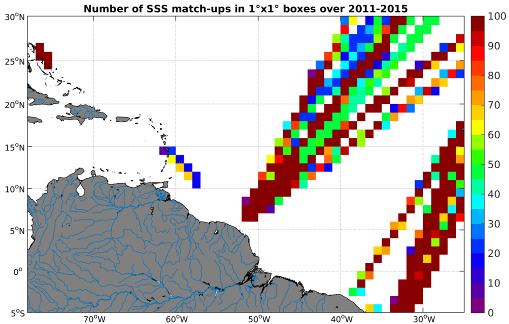
Figure 4: Number of SSS match-ups between TSG-LEGOS-DM SSS and the Aquarius-L4-IPRC-V4-MONTHLY SSS product for the Amazon and Orinoco river plumes Pi-MEP region over 1^\circ \times 1^\circ boxes and for the full satellite product period.
