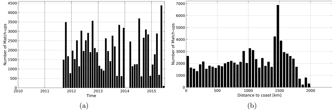
Figure 1: Number of match-ups between TSG-LEGOS-DM and Aquarius-L4-IPRC-V4-MONTHLY SSS as a function of time (a) and as function of the distance to coast (b) over the Amazon and Orinoco river plumes Pi-MEP region and for the full satellite product period.
