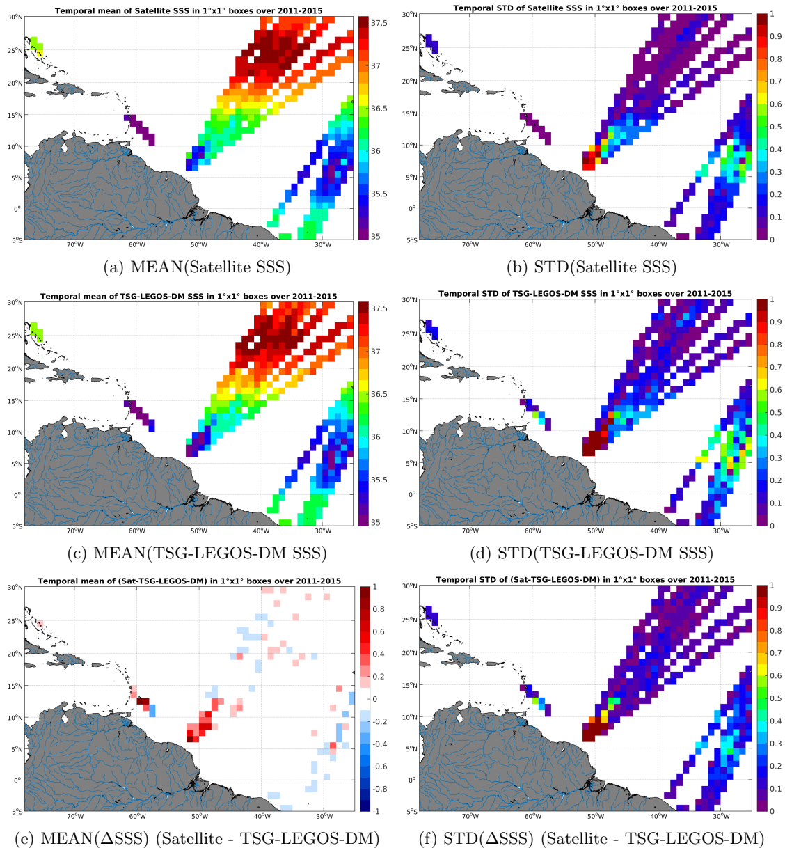
Figure 6: Temporal mean (left) and STD (right) of SSS from Aquarius-L4-IPRC-V4-MONTHLY (top), TSG-LEGOS-DM (middle), and of \Delta SSS (Satellite - TSG-LEGOS-DM). Only match-up pairs are used to generate these maps.
