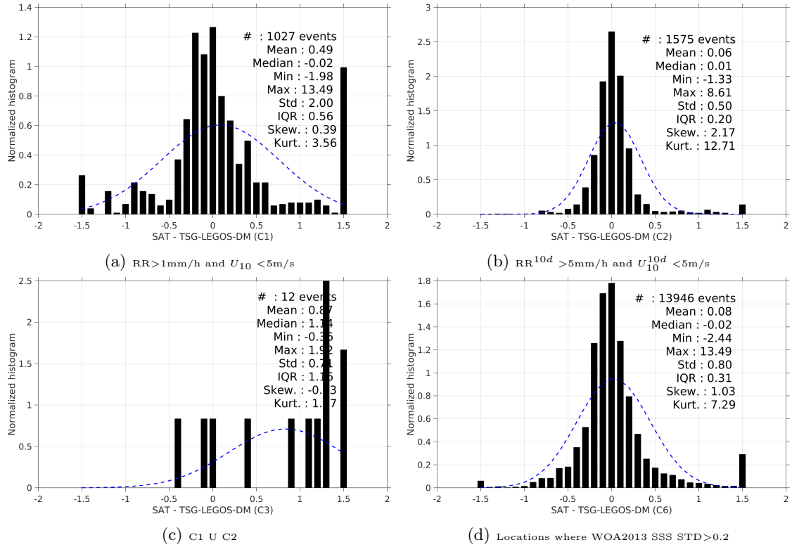
Figure 13: Normalized histogram of \Delta SSS (Aquarius-L4-IPRC-V4-MONTHLY - TSG-LEGOS-DM) for 6 different subdatasets corresponding to: RR > 1mm/h and U_{10} < 5 m/s (a), RR^{10d} > 5 mm/h and U_{10}^{10d} < 5 m/s (b), C1 U C2 (c), Locations where WOA2013 SSS STD > 0.2 (d).
