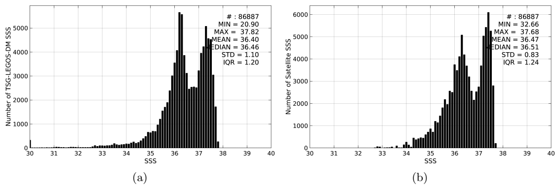
Figure 2: Histograms of SSS from TSG-LEGOS-DM (a) and Aquarius-L4-IPRC-V4-MONTHLY (b) considering all match-up pairs per bins of 0.1 over the Amazon and Orinoco river plumes Pi-MEP region and for the full satellite product period.
