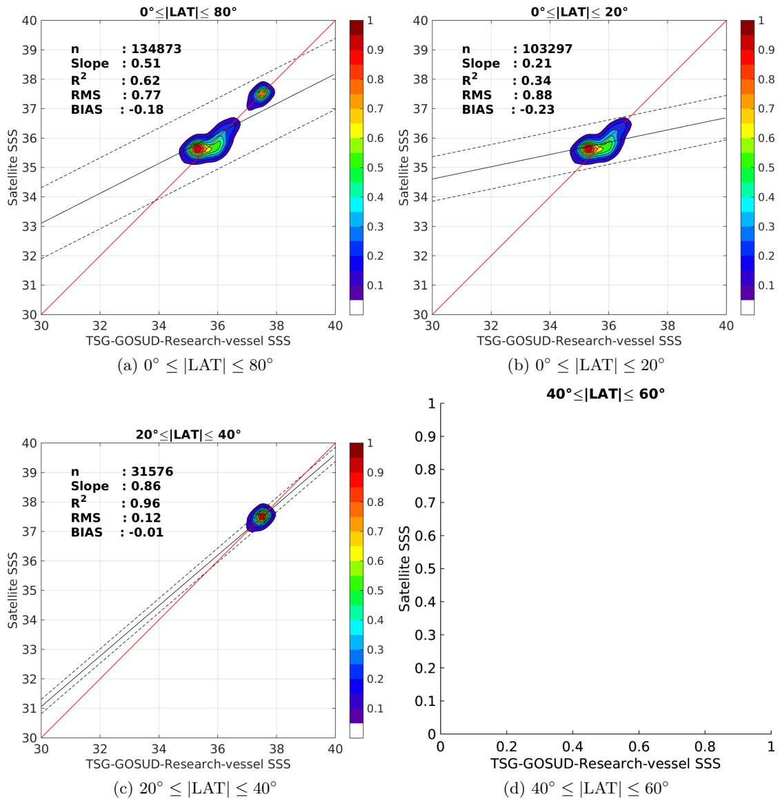
Figure 9: Contour maps of the concentration of Aquarius-L4-IPRC-V4-MONTHLY SSS (y-axis) versus TSG-GOSUD-Research-vessel SSS (x-axis) at match-up pairs for different latitude bands. For each plot, the red line shows x=y . The black thin and dashed lines indicate a linear fit through the data cloud and the \pm 95\% confidence levels, respectively. The number match-up pairs n , the slope and R^2 coefficient of the linear fit, the root mean square (RMS) and the mean bias between satellite and in situ data are indicated for each latitude band in each plots.
