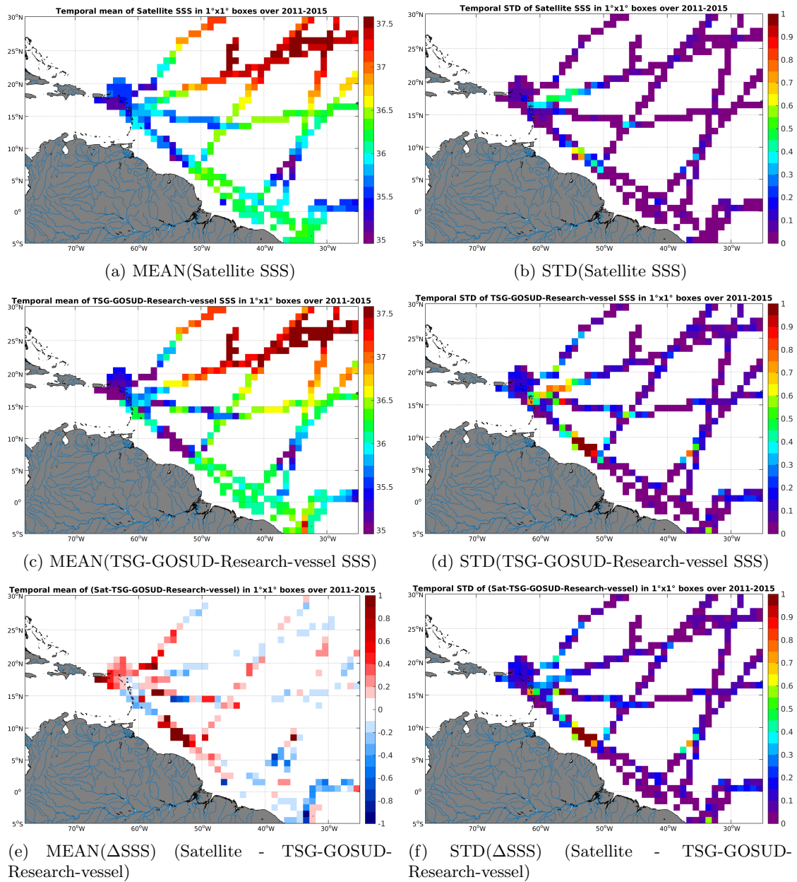
Figure 6: Temporal mean (left) and STD (right) of SSS from Aquarius-L4-IPRC-V4-MONTHLY (top), TSG-GOSUD-Research-vessel (middle), and of \Delta SSS (Satellite - TSG-GOSUD-Research-vessel). Only match-up pairs are used to generate these maps.
