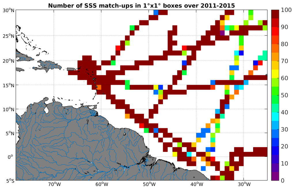
Figure 4: Number of SSS match-ups between TSG-GOSUD-Research-vessel SSS and the Aquarius-L4-IPRC-V4-MONTHLY SSS product for the Amazon and Orinoco river plumes Pi-MEP region over 1^\circ \times 1^\circ boxes and for the full satellite product period.
