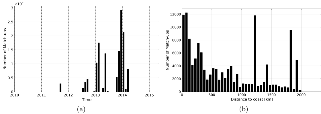
Figure 1: Number of match-ups between TSG-GOSUD-Research-vessel and Aquarius-L4-IPRC-V4-MONTHLY SSS as a function of time (a) and as function of the distance to coast (b) over the Amazon and Orinoco river plumes Pi-MEP region and for the full satellite product period.
