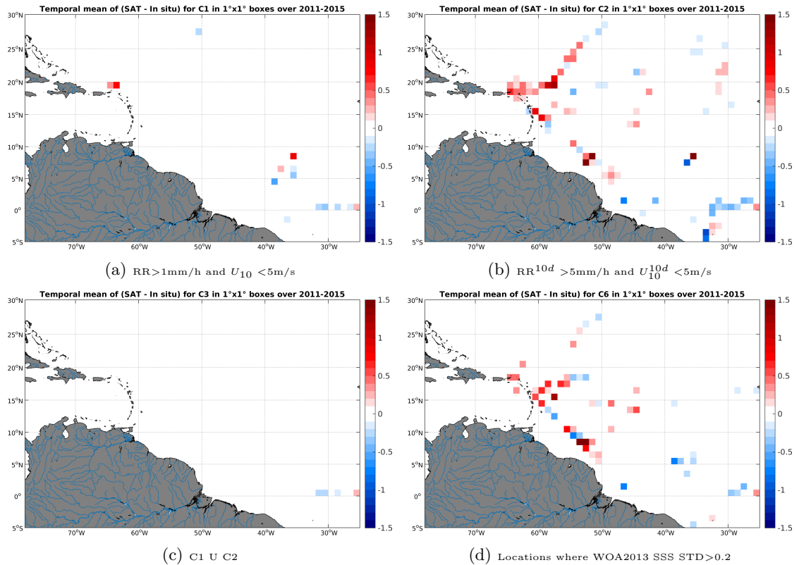
Figure 12: Temporal mean gridded over spatial boxes of size 1^\circ \times 1^\circ of \Delta SSS (Aquarius-L4-IPRC-V4-MONTHLY - TSG-GOSUD-Research-vessel) for 4 different subdatasets corresponding to:RR > 1 mm/h and U_{10} < 5 m/s (a), RR^{10d} > 5 mm/h and U_{10}^{10d} < 5 m/s (b), C1 U C2 (c),Locations where WOA2013 SSS STD > 0.2 (d).
