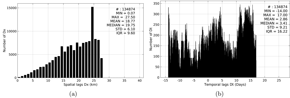
Figure 5: Histograms of the spatial (a) and temporal (b) lags between the time of the TSG-GOSUD-Research-vessel measurements and the date of the corresponding Aquarius-L4-IPRC-V4-MONTHLY SSS product.
