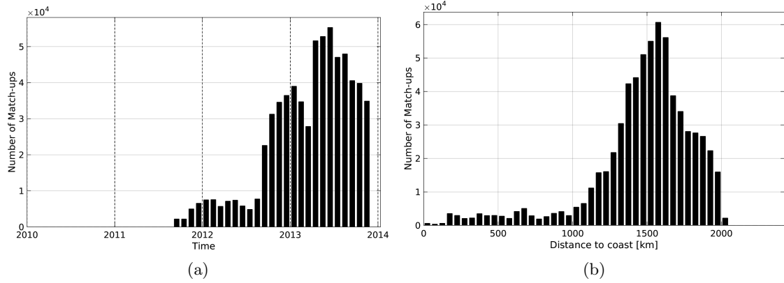
Figure 1: Number of match-ups between Surface drifters and Aquarius-L4-IPRC-V4-MONTHLY SSS as a function of time (a) and as function of the distance to coast (b) over the Amazon and Orinoco river plumes Pi-MEP region and for the full satellite product period.
