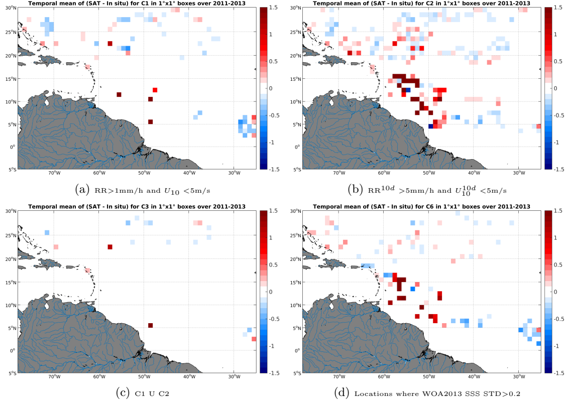
Figure 11: Temporal mean gridded over spatial boxes of size 1^\circ \times 1^\circ of \Delta SSS (Aquarius-L4-IPRC-V4-MONTHLY - Surface drifters) for 4 different subdatasets corresponding to: RR > 1mm/h and U_{10} < 5 m/s (a), RR^{10d} > 5 mm/h and U_{10}^{10d} < 5 m/s (b), C1 U C2 (c), Locations where WOA2013 SSS STD > 0.2 (d).
