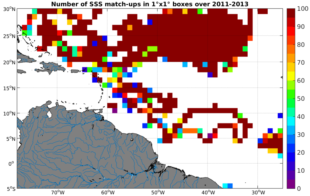
Figure 3: Number of SSS match-ups between Surface drifters SSS and the Aquarius-L4-IPRC-V4-MONTHLY SSS product for the Amazon and Orinoco river plumes Pi-MEP region over 1^\circ \times 1^\circ boxes and for the full satellite product period.
