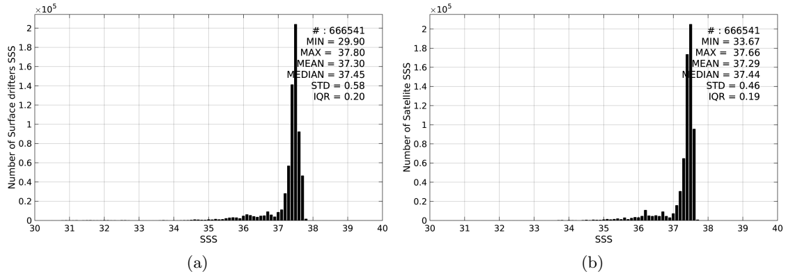
Figure 2: Histograms of SSS from Surface drifters (a) and Aquarius-L4-IPRC-V4-MONTHLY (b) considering all match-up pairs per bins of 0.1 over the Amazon and Orinoco river plumes Pi-MEP region and for the full satellite product period.
