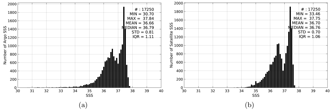
Figure 2: Histograms of SSS from Argo (a) and Aquarius-L4-IPRC-V4-MONTHLY (b) considering all match-up pairs per bins of 0.1 over the Amazon and Orinoco river plumes Pi-MEP region and for the full satellite product period.
