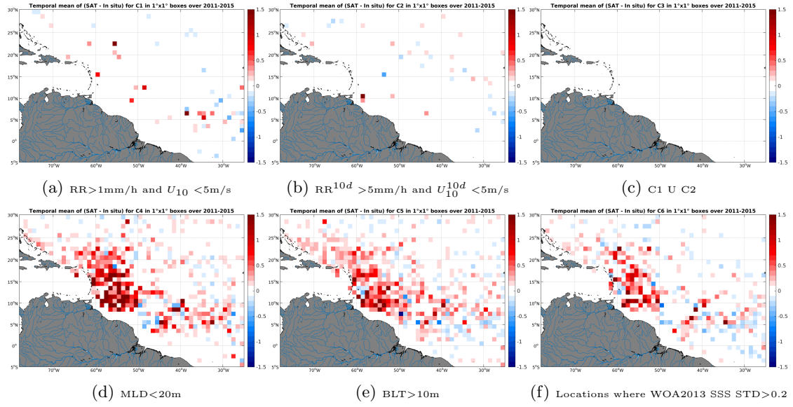
Figure 12: Temporal mean gridded over spatial boxes of size 1^\circ \times 1^\circ of \Delta SSS (Aquarius-L4-IPRC-V4-MONTHLY - Argo) for 6 different subdatasets corresponding to: RR > 1\text{mm/h} and U_{10} < 5\text{m/s} (a), RR^{10d} > 5\text{mm/h} and U_{10}^{10d} < 5\text{m/s} (b), C1 U C2 (c), MLD < 20\text{m} (d), BLT > 10\text{m} (e), Locations where WOA2013 SSS STD > 0.2 (f).
