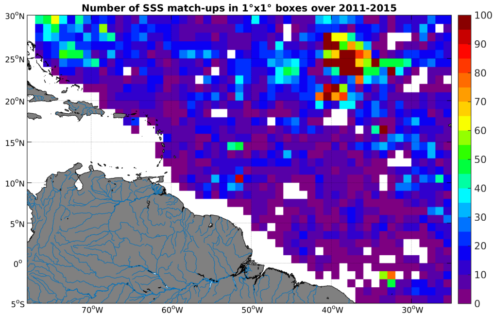
Figure 4: Number of SSS match-ups between Argo SSS and the Aquarius-L4-IPRC-V4-MONTHLY SSS product for the Amazon and Orinoco river plumes Pi-MEP region over 1^\circ \times 1^\circ boxes and for the full satellite product period.
