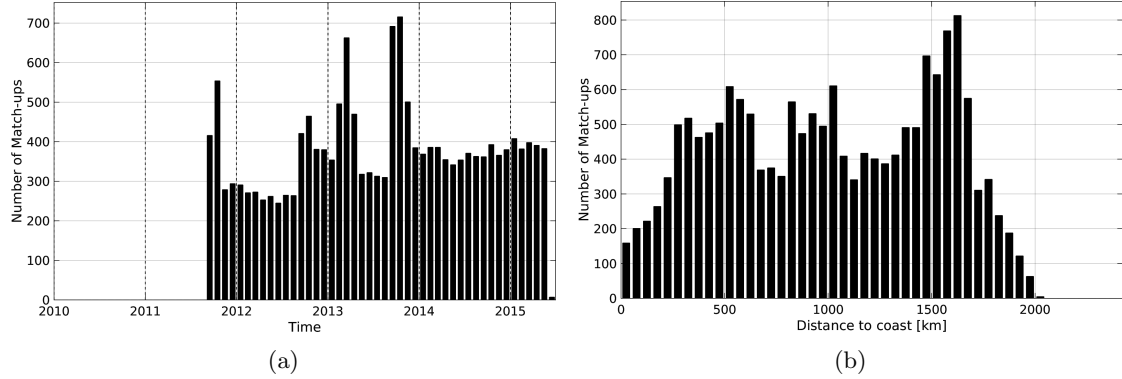
Figure 1: Number of match-ups between Argo and Aquarius-L4-IPRC-V4-MONTHLY SSS as a function of time (a) and as function of the distance to coast (b) over the Amazon and Orinoco river plumes Pi-MEP region and for the full satellite product period.
