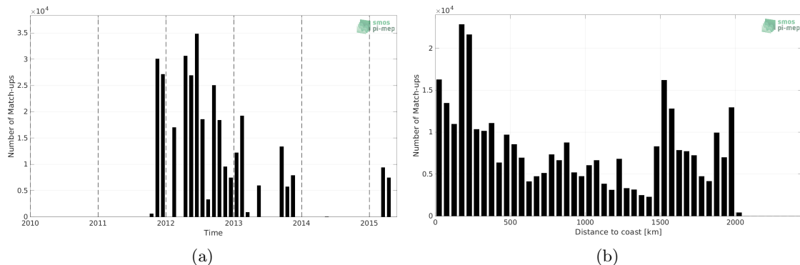
Figure 1: Number of match-ups between TSG (SAMOS) and Aquarius SSS L3 OR v5 - 7-Day running (NASA-GSFC) SSS as a function of time (a) and as function of the distance to coast (b) over the Amazon and Orinoco river plumes Pi-MEP region and for the full satellite product period.
