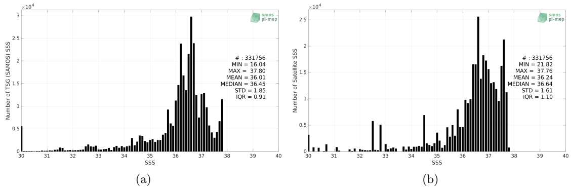
Figure 2: Histograms of SSS from TSG (SAMOS) (a) and Aquarius SSS L3 OR v5 - 7-Day running (NASA-GSFC) (b) considering all match-up pairs per bins of 0.1 over the Amazon and Orinoco river plumes Pi-MEP region and for the full satellite product period.
