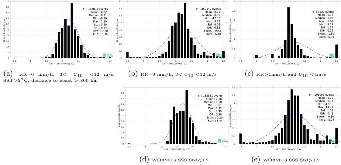
Figure 13: Normalized histogram of \Delta SSS (Aquarius SSS L3 OR v5 - 7-Day running (NASA-GSFC) - TSG (SAMOS)) for 5 different subdatasets corresponding to: RR=0 mm/h, 3 < U_{10} < 12 m/s, SST>5°C, distance to coast > 800 km (a), RR=0 mm/h, 3 < U_{10} < 12 m/s (b), RR>1mm/h and U_{10} < 4 m/s (c), WOA2013 SSS Std<0.2 (d), WOA2013 SSS Std>0.2 (e).
