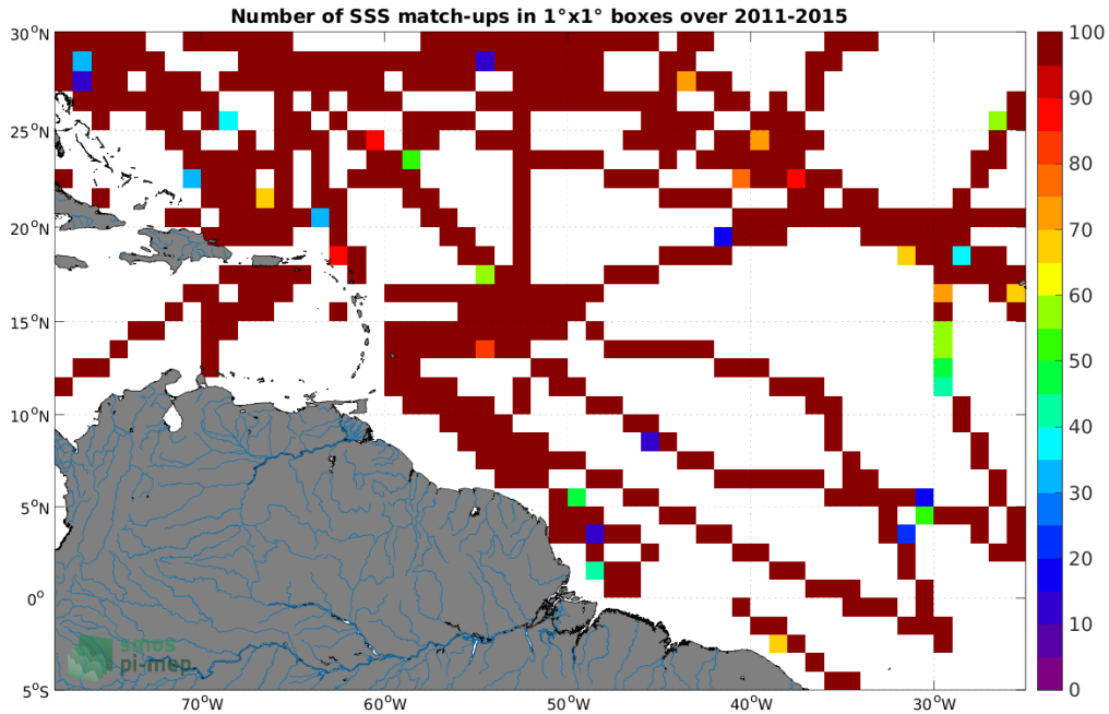
Figure 4: Number of SSS match-ups between TSG (SAMOS) SSS and the Aquarius SSS L3 OR v5 - 7-Day running (NASA-GSFC) SSS product for the Amazon and Orinoco river plumes Pi-MEP region over 1^\circ \times 1^\circ boxes and for the full satellite product period.
