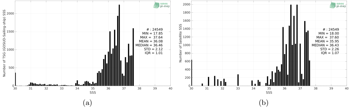
Figure 2: Histograms of SSS from TSG (GOSUD-Sailing-ship) (a) and Aquarius SSS L3 OR v5 - 7-Day running (NASA-GSFC) (b) considering all match-up pairs per bins of 0.1 over the Amazon and Orinoco river plumes Pi-MEP region and for the full satellite product period.
