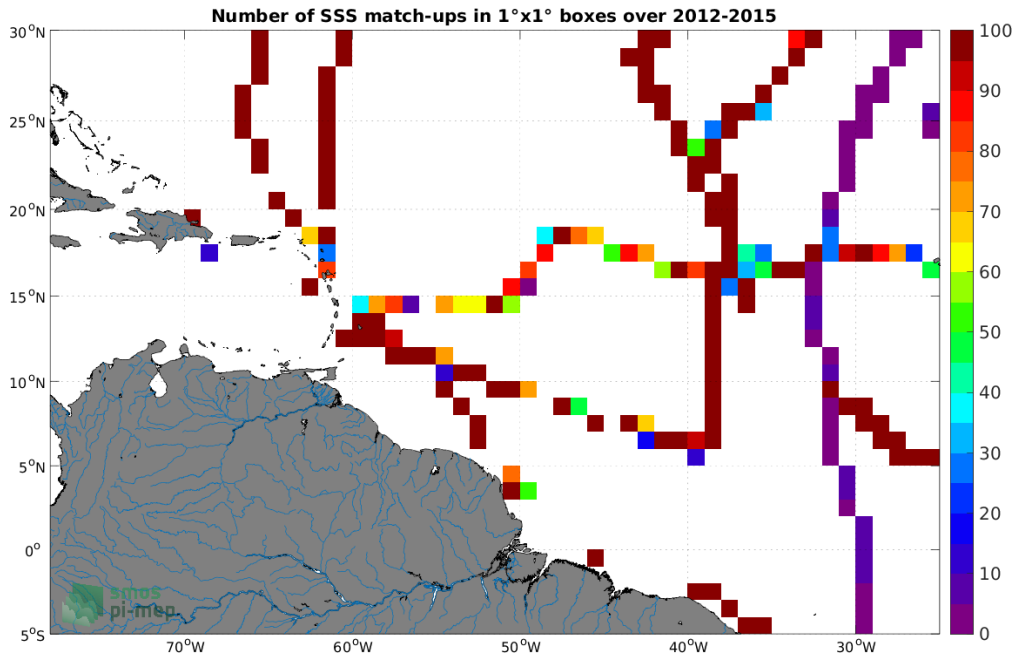
Figure 4: Number of SSS match-ups between TSG (GOSUD-Sailing-ship) SSS and the Aquarius SSS L3 OR v5 - 7-Day running (NASA-GSFC) SSS product for the Amazon and Orinoco river plumes Pi-MEP region over 1^\circ \times 1^\circ boxes and for the full satellite product period.
