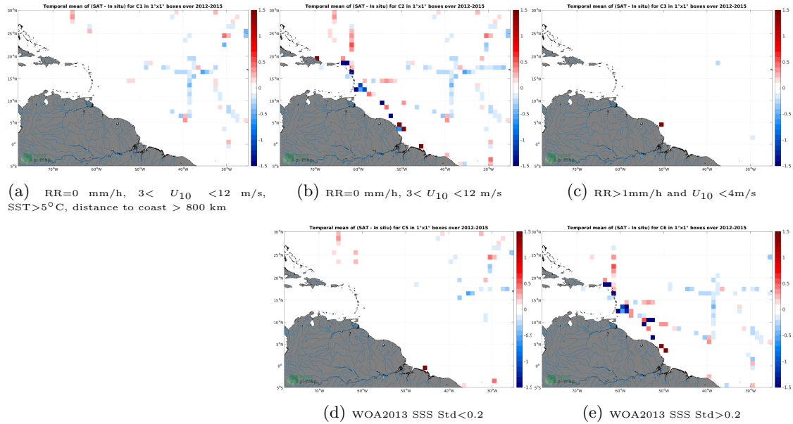
Figure 12: Temporal mean gridded over spatial boxes of size 1^{\circ}\times 1^{\circ} of \Delta SSS (Aquarius SSS L3 OR v5 - 7-Day running (NASA-GSFC) - TSG (GOSUD-Sailing-ship)) for 5 different subdatasets corresponding to:RR=0 mm/h, 3 < U_{10} < 12 m/s, SST >5^{\circ}\text{C} , distance to coast > 800 km (a), RR=0 mm/h, 3 < U_{10} < 12 m/s (b), RR >1 mm/h and U_{10} < 4 m/s (c), WOA2013 SSS Std <0.2 (d), WOA2013 SSS Std >0.2 (e).
