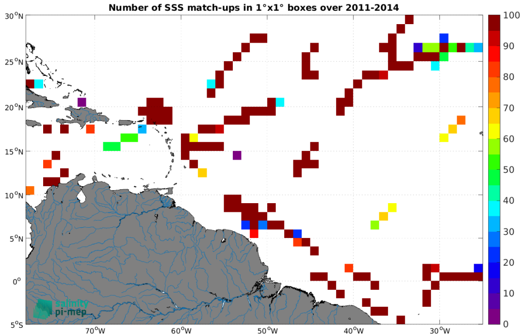
Figure 5: Number of SSS match-ups between TSG (GOSUD-Research-vessel) SSS and the Aquarius SSS L3 OR v5 - 7-Day running (NASA-GSFC) SSS product for the Amazon and Orinoco river plumes Pi-MEP region over 1^\circ \times 1^\circ boxes and for the full satellite product period.
