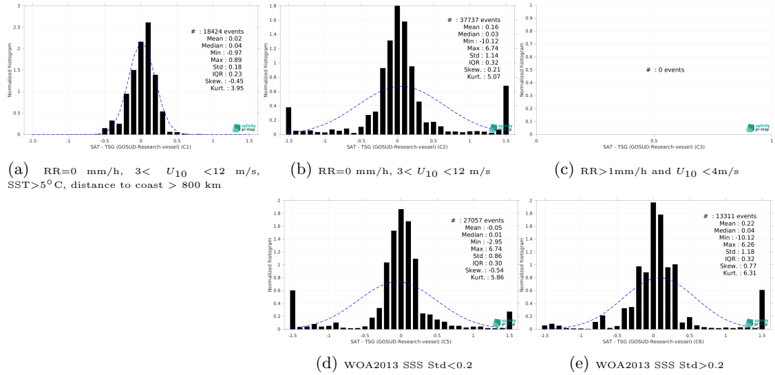
Figure 15: Normalized histogram of \Delta SSS (Aquarius SSS L3 OR v5 - 7-Day running (NASA-GSFC) - TSG (GOSUD-Research-vessel)) for 5 different subdatasets corresponding to: RR=0 mm/h, 3 < U_{10} < 12 m/s, SST > 5°C, distance to coast > 800 km (a), RR=0 mm/h, 3 < U_{10} < 12 m/s (b), RR > 1mm/h and U_{10} < 4 m/s (c), WOA2013 SSS Std < 0.2 (d), WOA2013 SSS Std > 0.2 (e).
