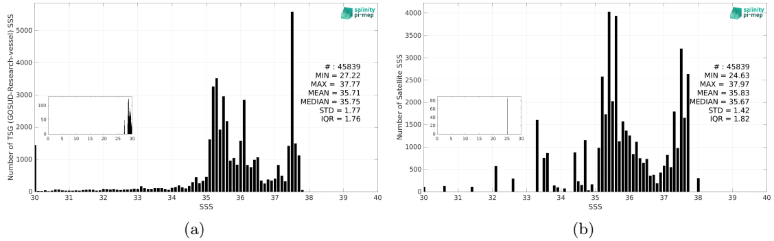
Figure 3: Histograms of SSS from TSG (GOSUD-Research-vessel) (a) and Aquarius SSS L3 OR v5 - 7-Day running (NASA-GSFC) (b) considering all match-up pairs per bins of 0.1 over the Amazon and Orinoco river plumes Pi-MEP region and for the full satellite product period.
