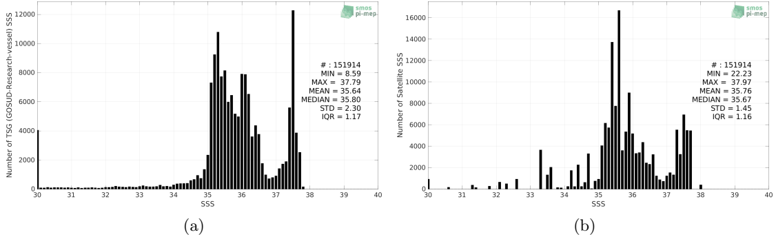
Figure 2: Histograms of SSS from TSG (GOSUD-Research-vessel) (a) and Aquarius SSS L3 OR v5 - 7-Day running (NASA-GSFC) (b) considering all match-up pairs per bins of 0.1 over the Amazon and Orinoco river plumes Pi-MEP region and for the full satellite product period.
