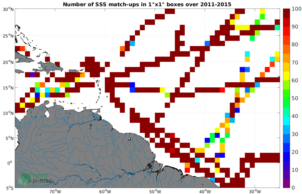
Figure 4: Number of SSS match-ups between TSG (GOSUD-Research-vessel) SSS and the Aquarius SSS L3 OR v5 - 7-Day running (NASA-GSFC) SSS product for the Amazon and Orinoco river plumes Pi-MEP region over 1^\circ \times 1^\circ boxes and for the full satellite product period.
