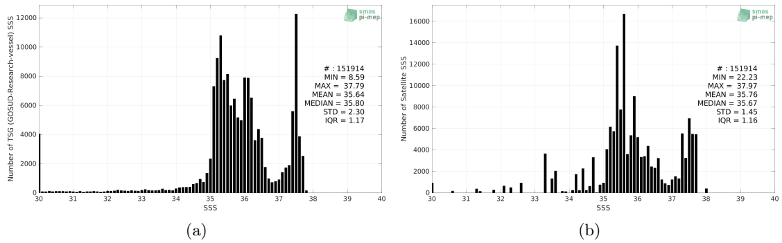
Figure 2: Histograms of SSS from TSG (GOSUD-Research-vessel) (a) and Aquarius SSS L3 OR v5 - 7-Day running (NASA-GSFC) (b) considering all match-up pairs per bins of 0.1 over the Amazon and Orinoco river plumes Pi-MEP region and for the full satellite product period.
