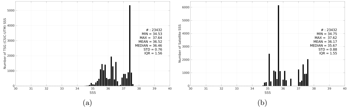
Figure 3: Histograms of SSS from TSG (CSIC-UTM) (a) and Aquarius SSS L3 OR v5 - 7-Day running (NASA-GSFC) (b) considering all match-up pairs per bins of 0.1 over the Amazon and Orinoco river plumes Pi-MEP region and for the full satellite product period.
