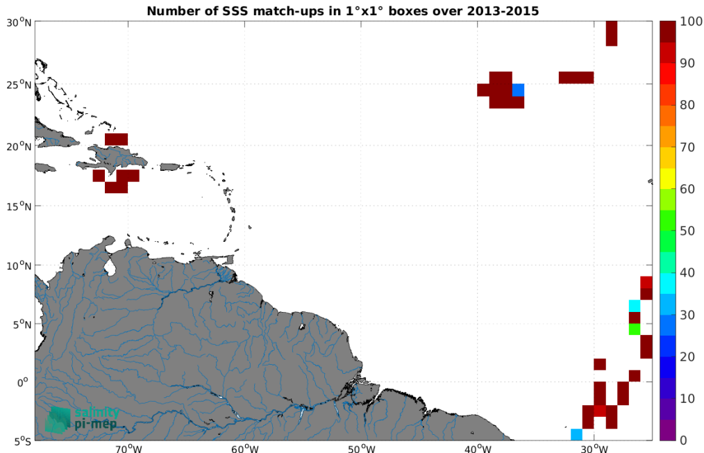
Figure 5: Number of SSS match-ups between TSG (CSIC-UTM) SSS and the Aquarius SSS L3 OR v5 - 7-Day running (NASA-GSFC) SSS product for the Amazon and Orinoco river plumes Pi-MEP region over 1^\circ \times 1^\circ boxes and for the full satellite product period.
