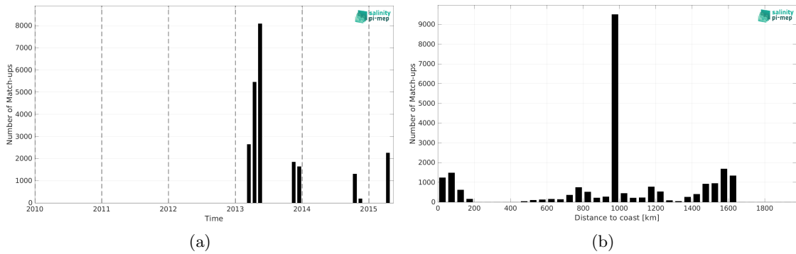
Figure 2: Number of match-ups between TSG (CSIC-UTM) and Aquarius SSS L3 OR v5 - 7-Day running (NASA-GSFC) SSS as a function of time (a) and as function of the distance to coast (b) over the Amazon and Orinoco river plumes Pi-MEP region and for the full satellite product period.
