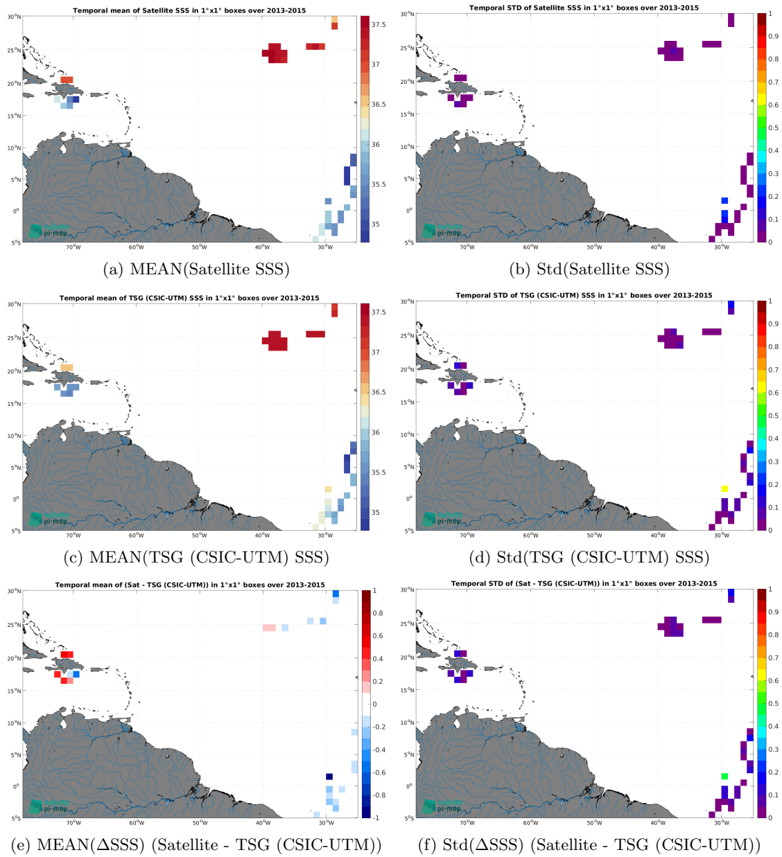
Figure 7: Temporal mean (left) and Std (right) of SSS from Aquarius SSS L3 OR v5 - 7-Day running (NASA-GSFC) (top), TSG (CSIC-UTM) (middle), and of \Delta SSS (Satellite - TSG (CSIC-UTM)). Only match-up pairs are used to generate these maps.
