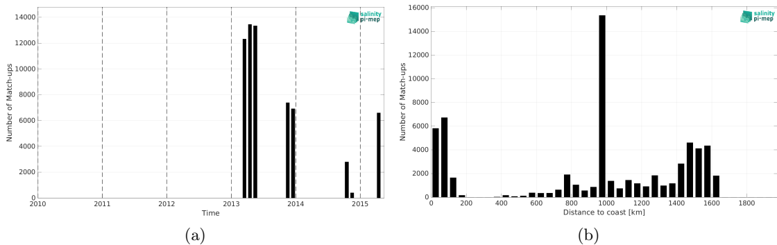
Figure 1: Number of match-ups between TSG (CSIC-UTM) and Aquarius SSS L3 OR v5 - 7-Day running (NASA-GSFC) SSS as a function of time (a) and as function of the distance to coast (b) over the Amazon and Orinoco river plumes Pi-MEP region and for the full satellite product period.
