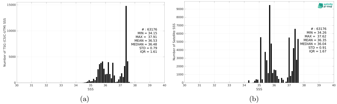
Figure 2: Histograms of SSS from TSG (CSIC-UTM) (a) and Aquarius SSS L3 OR v5 - 7-Day running (NASA-GSFC) (b) considering all match-up pairs per bins of 0.1 over the Amazon and Orinoco river plumes Pi-MEP region and for the full satellite product period.
