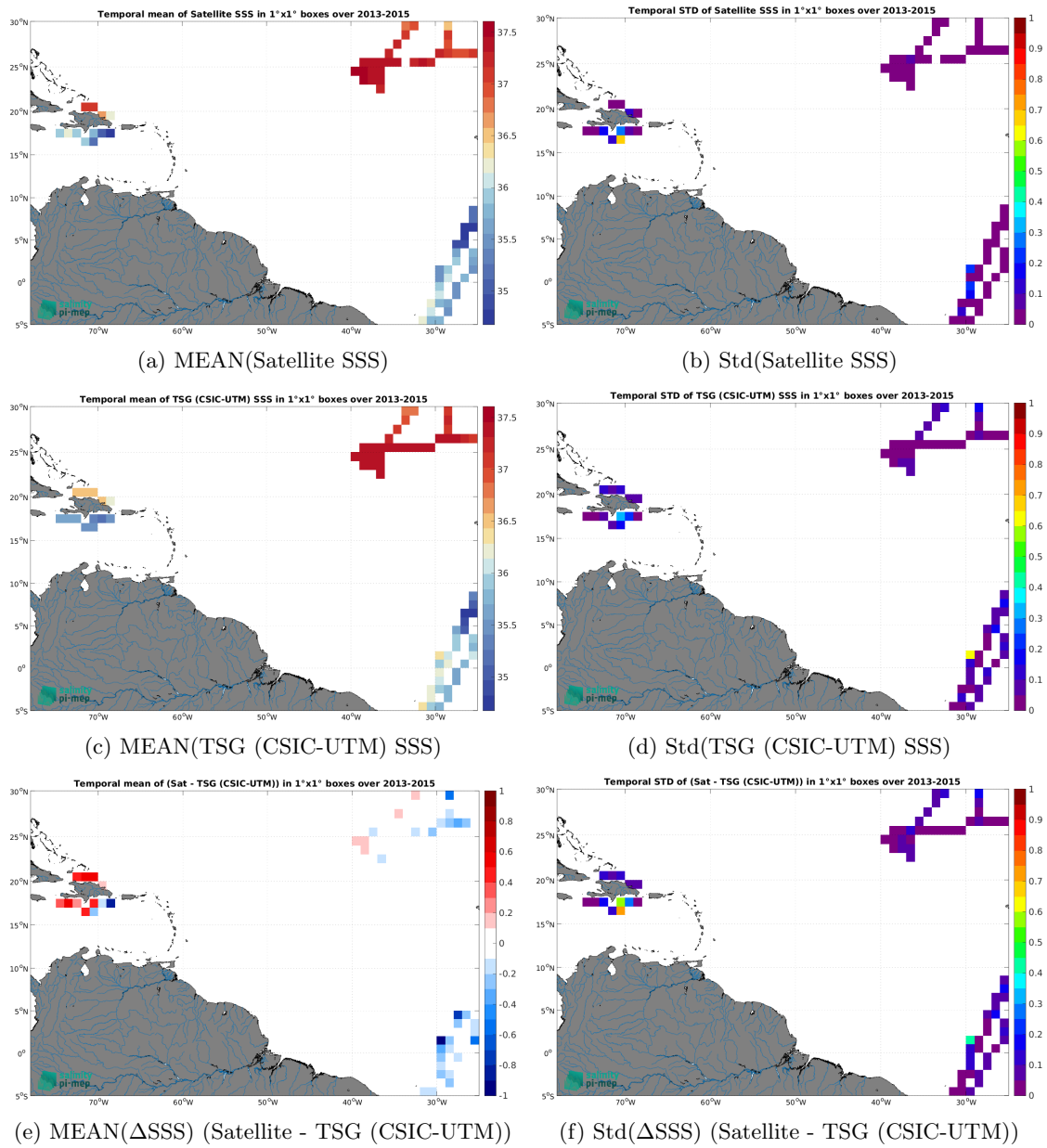
Figure 6: Temporal mean (left) and Std (right) of SSS from Aquarius SSS L3 OR v5 - 7-Day running (NASA-GSFC) (top), TSG (CSIC-UTM) (middle), and of \Delta SSS (Satellite - TSG (CSIC-UTM)). Only match-up pairs are used to generate these maps.
