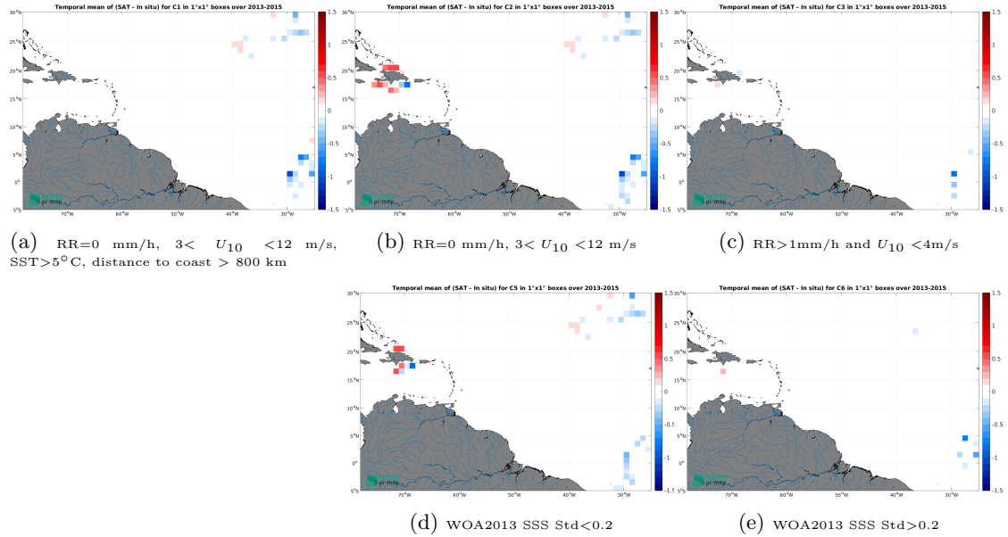
Figure 12: Temporal mean gridded over spatial boxes of size 1^{\circ}\times 1^{\circ} of \Delta\text{SSS} (Aquarius SSS L3 OR v5 - 7-Day running (NASA-GSFC) - TSG (CSIC-UTM)) for 5 different subdatasets corresponding to:RR=0 mm/h, 3 < U_{10} < 12 m/s, SST >5^{\circ}\text{C} , distance to coast > 800 km (a), RR=0 mm/h, 3 < U_{10} < 12 m/s (b), RR >1 mm/h and U_{10} < 4 m/s (c), WOA2013 SSS Std <0.2 (d), WOA2013 SSS Std >0.2 (e).
