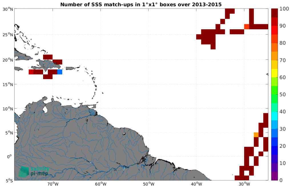
Figure 4: Number of SSS match-ups between TSG (CSIC-UTM) SSS and the Aquarius SSS L3 OR v5 - 7-Day running (NASA-GSFC) SSS product for the Amazon and Orinoco river plumes Pi-MEP region over 1^\circ \times 1^\circ boxes and for the full satellite product period.
