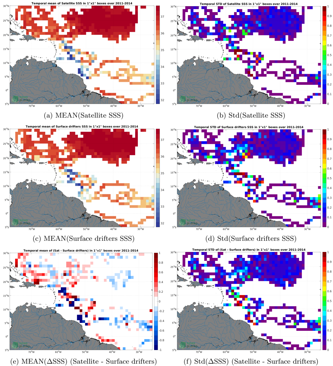
Figure 5: Temporal mean (left) and Std (right) of SSS from Aquarius SSS L3 OR v5 - 7-Day running (NASA-GSFC) (top), Surface drifters (middle), and of \Delta SSS (Satellite - Surface drifters). Only match-up pairs are used to generate these maps.
