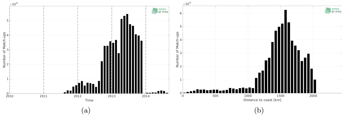
Figure 1: Number of match-ups between Surface drifters and Aquarius SSS L3 OR v5 - 7-Day running (NASA-GSFC) SSS as a function of time (a) and as function of the distance to coast (b) over the Amazon and Orinoco river plumes Pi-MEP region and for the full satellite product period.
