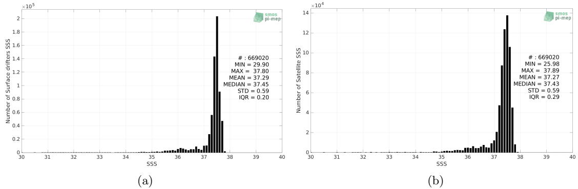
Figure 2: Histograms of SSS from Surface drifters (a) and Aquarius SSS L3 OR v5 - 7-Day running (NASA-GSFC) (b) considering all match-up pairs per bins of 0.1 over the Amazon and Orinoco river plumes Pi-MEP region and for the full satellite product period.
