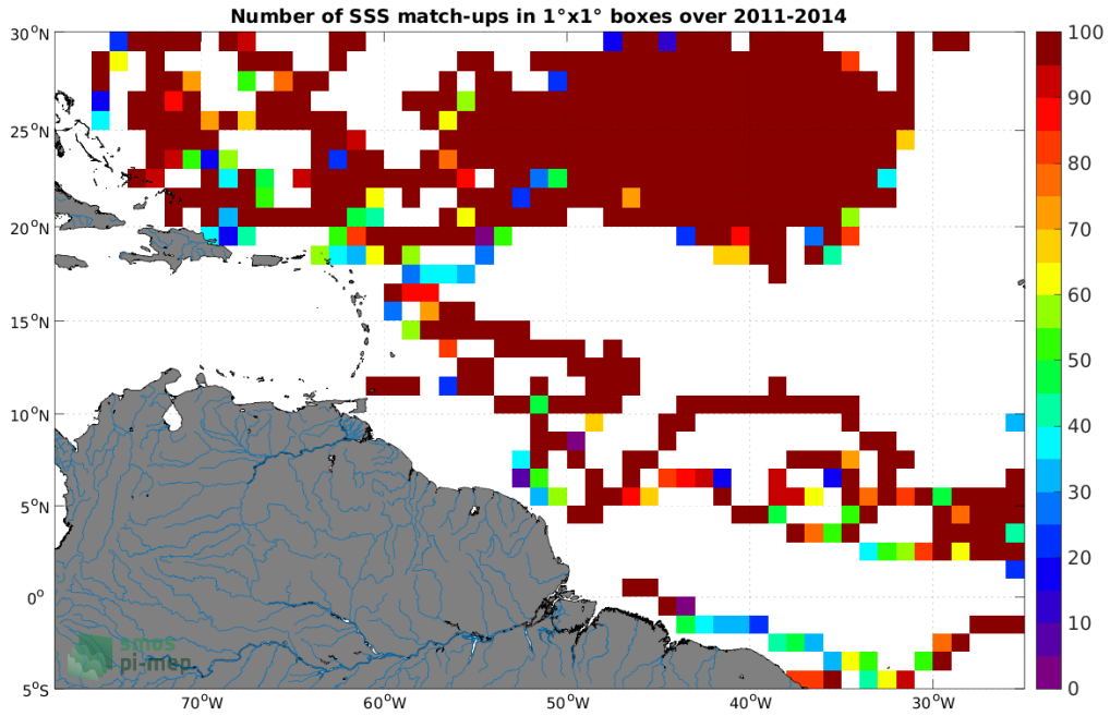
Figure 3: Number of SSS match-ups between Surface drifters SSS and the Aquarius SSS L3 OR v5 - 7-Day running (NASA-GSFC) SSS product for the Amazon and Orinoco river plumes Pi-MEP region over 1^\circ \times 1^\circ boxes and for the full satellite product period.
