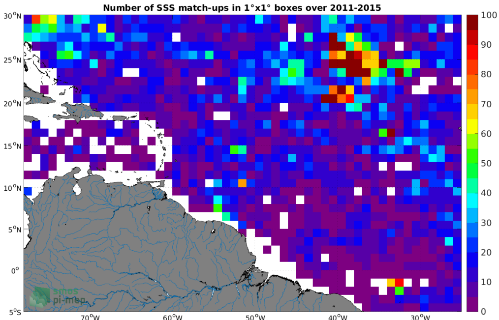
Figure 4: Number of SSS match-ups between Argo SSS and the Aquarius SSS L3 OR v5 - 7-Day running (NASA-GSFC) SSS product for the Amazon and Orinoco river plumes Pi-MEP region over 1^\circ \times 1^\circ boxes and for the full satellite product period.
