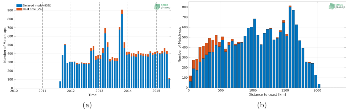
Figure 1: Number of match-ups between Argo and Aquarius SSS L3 OR v5 - 7-Day running (NASA-GSFC) SSS as a function of time (a) and as function of the distance to coast (b) over the Amazon and Orinoco river plumes Pi-MEP region and for the full satellite product period.
