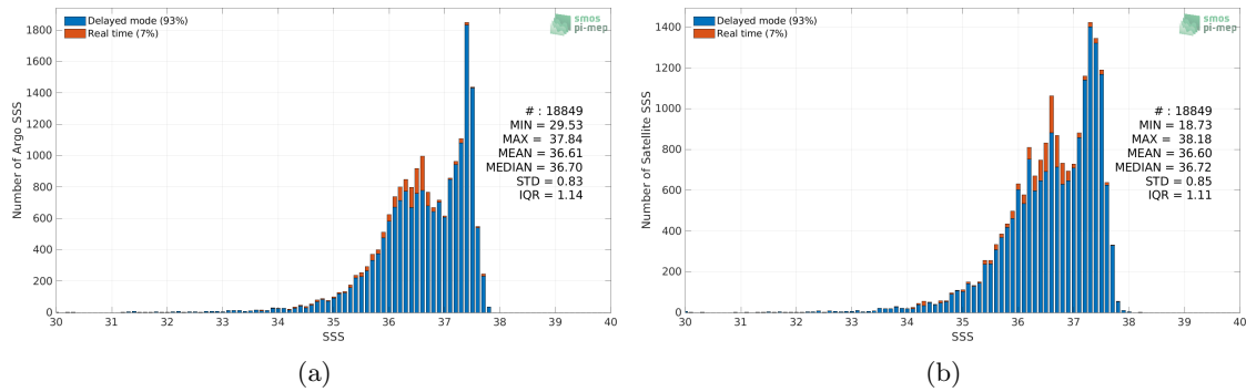
Figure 2: Histograms of SSS from Argo (a) and Aquarius SSS L3 OR v5 - 7-Day running (NASA-GSFC) (b) considering all match-up pairs per bins of 0.1 over the Amazon and Orinoco river plumes Pi-MEP region and for the full satellite product period.
