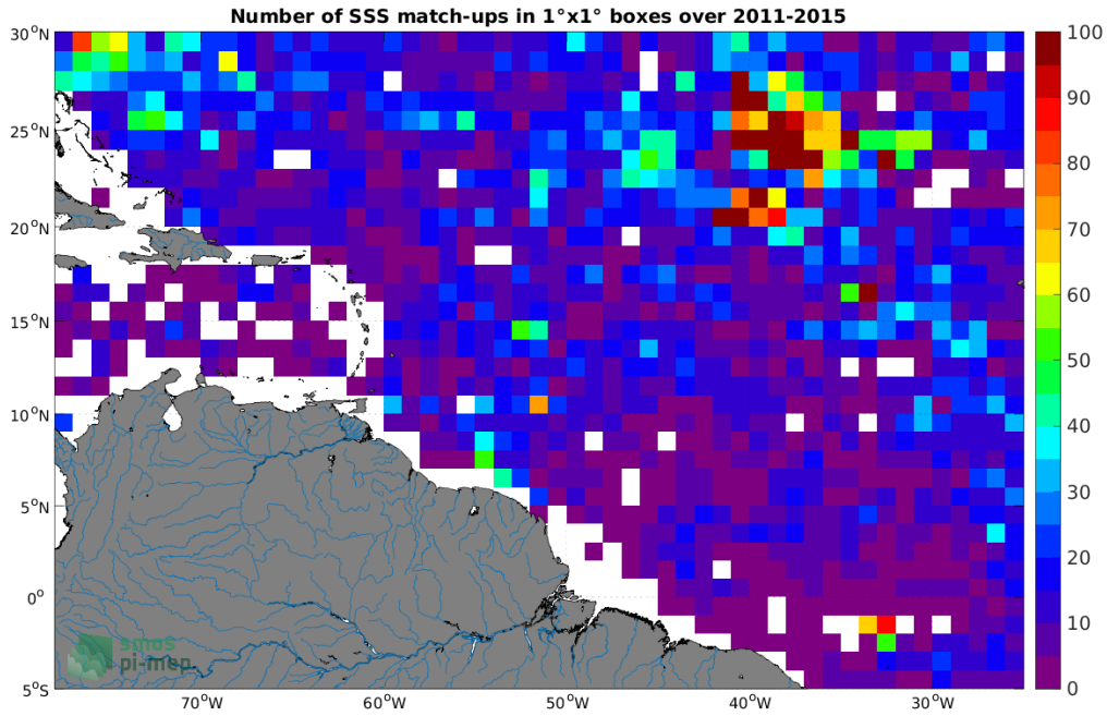
Figure 4: Number of SSS match-ups between Argo SSS and the Aquarius SSS L3 OR v5 - 7-Day running (NASA-GSFC) SSS product for the Amazon and Orinoco river plumes Pi-MEP region over 1^{\circ} \times 1^{\circ} boxes and for the full satellite product period.
