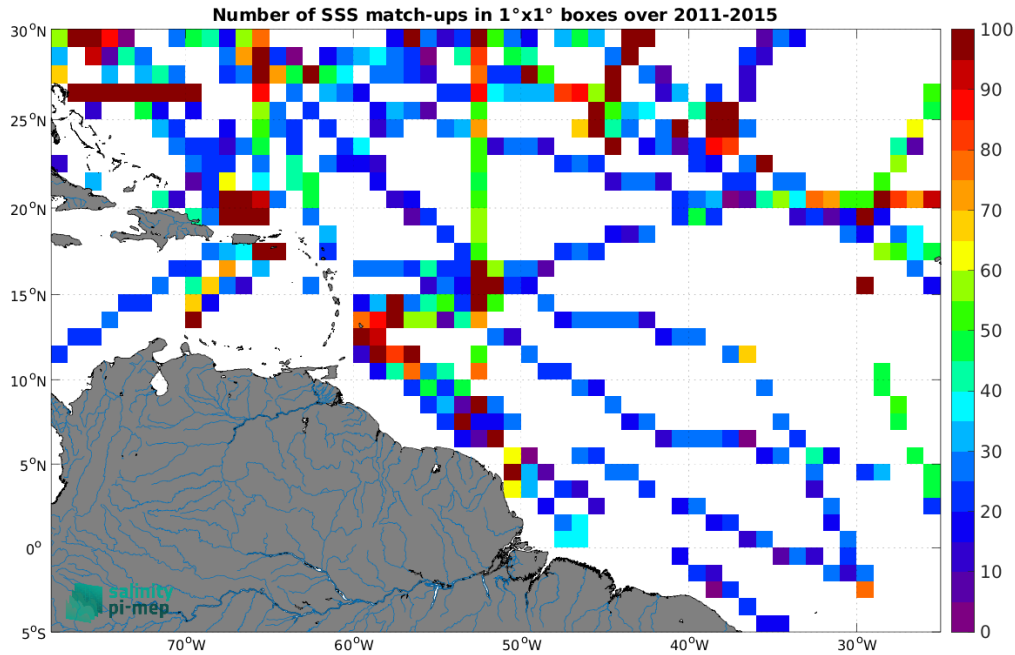
Figure 5: Number of SSS match-ups between TSG (SAMOS) SSS and the Aquarius SSS L3 OR v5 - 7-Day running - Rain mask (NASA-GSFC) SSS product for the Amazon and Orinoco river plumes Pi-MEP region over 1^\circ \times 1^\circ boxes and for the full satellite product period.
