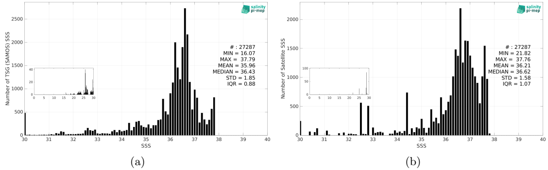
Figure 3: Histograms of SSS from TSG (SAMOS) (a) and Aquarius SSS L3 OR v5 - 7-Day running - Rain mask (NASA-GSFC) (b) considering all match-up pairs per bins of 0.1 over the Amazon and Orinoco river plumes Pi-MEP region and for the full satellite product period.
