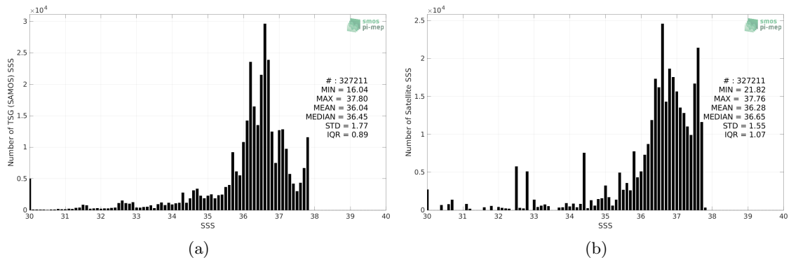
Figure 2: Histograms of SSS from TSG (SAMOS) (a) and Aquarius SSS L3 OR v5 - 7-Day running - Rain mask (NASA-GSFC) (b) considering all match-up pairs per bins of 0.1 over the Amazon and Orinoco river plumes Pi-MEP region and for the full satellite product period.
