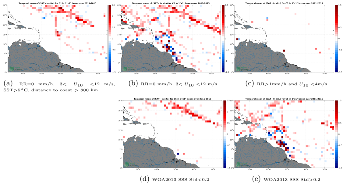
Figure 12: Temporal mean gridded over spatial boxes of size 1^{\circ}\times 1^{\circ} of \Delta\text{SSS} (Aquarius SSS L3 OR v5 - 7-Day running - Rain mask (NASA-GSFC) - TSG (SAMOS)) for 5 different subdatasets corresponding to:RR=0 mm/h, 3 < U_{10} < 12 m/s, SST >5^{\circ}\text{C} , distance to coast > 800 km (a), RR=0 mm/h, 3 < U_{10} < 12 m/s (b), RR >1 mm/h and U_{10} < 4 m/s (c), WOA2013 SSS Std <0.2 (d), WOA2013 SSS Std >0.2 (e).
