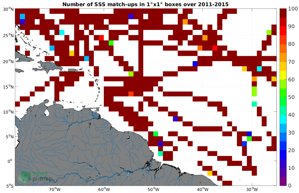
Figure 4: Number of SSS match-ups between TSG (SAMOS) SSS and the Aquarius SSS L3 OR v5 - 7-Day running - Rain mask (NASA-GSFC) SSS product for the Amazon and Orinoco river plumes Pi-MEP region over 1^\circ \times 1^\circ boxes and for the full satellite product period.
