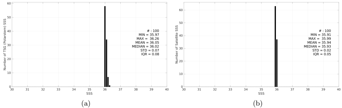
Figure 3: Histograms of SSS from TSG (Polarstern) (a) and Aquarius SSS L3 OR v5 - 7-Day running - Rain mask (NASA-GSFC) (b) considering all match-up pairs per bins of 0.1 over the Amazon and Orinoco river plumes Pi-MEP region and for the full satellite product period.
