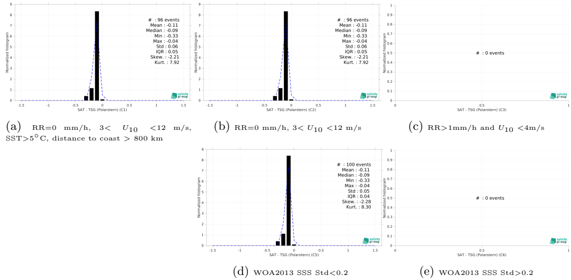
Figure 15: Normalized histogram of \Delta\text{SSS} (Aquarius SSS L3 OR v5 - 7-Day running - Rain mask (NASA-GSFC) - TSG (Polarstern)) for 5 different subdatasets corresponding to: RR=0 mm/h, 3 < U_{10} < 12 m/s, SST > 5^\circ\text{C} , distance to coast > 800 km (a), RR=0 mm/h, 3 < U_{10} < 12 m/s (b), RR > 1\text{mm/h} and U_{10} < 4\text{m/s} (c), WOA2013 SSS Std < 0.2 (d), WOA2013 SSS Std > 0.2 (e).
