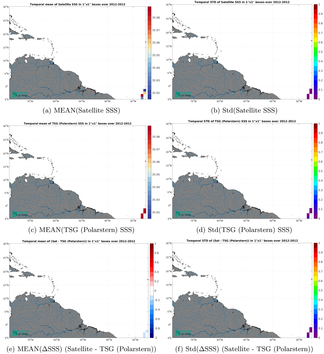
Figure 7: Temporal mean (left) and Std (right) of SSS from Aquarius SSS L3 OR v5 - 7-Day running - Rain mask (NASA-GSFC) (top), TSG (Polarstern) (middle), and of \Delta SSS (Satellite - TSG (Polarstern)). Only match-up pairs are used to generate these maps.
