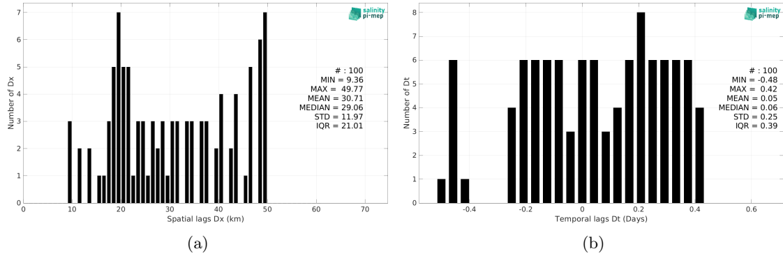
Figure 6: Histograms of the spatial (a) and temporal (b) lags between the location/time of the TSG (Polarstern) measurement and the date of the corresponding Aquarius SSS L3 OR v5 - 7-Day running - Rain mask (NASA-GSFC) SSS pixel.
