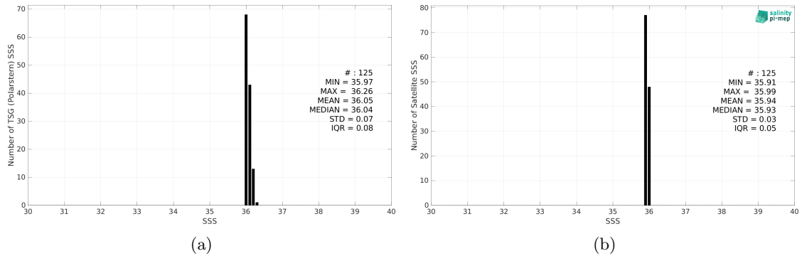
Figure 2: Histograms of SSS from TSG (Polarstern) (a) and Aquarius SSS L3 OR v5 - 7-Day running - Rain mask (NASA-GSFC) (b) considering all match-up pairs per bins of 0.1 over the Amazon and Orinoco river plumes Pi-MEP region and for the full satellite product period.
