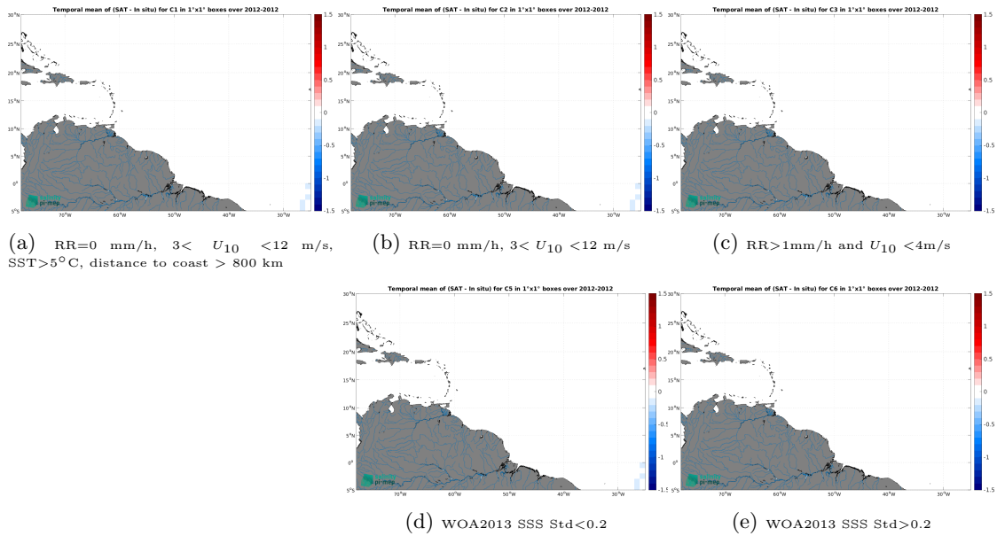
Figure 12: Temporal mean gridded over spatial boxes of size 1^{\circ}\times 1^{\circ} of \Delta\text{SSS} (Aquarius SSS L3 OR v5 - 7-Day running - Rain mask (NASA-GSFC) - TSG (Polarstern)) for 5 different subdatasets corresponding to:RR=0 mm/h, 3 < U_{10} < 12 m/s, SST > 5^{\circ}\text{C} , distance to coast > 800 km (a), RR=0 mm/h, 3 < U_{10} < 12 m/s (b), RR > 1 mm/h and U_{10} < 4 m/s (c), WOA2013 SSS Std < 0.2 (d), WOA2013 SSS Std > 0.2 (e).
