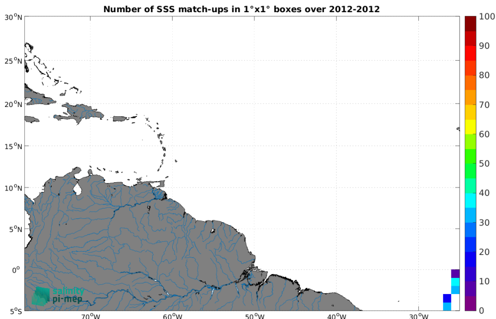
Figure 4: Number of SSS match-ups between TSG (Polarstern) SSS and the Aquarius SSS L3 OR v5 - 7-Day running - Rain mask (NASA-GSFC) SSS product for the Amazon and Orinoco river plumes Pi-MEP region over 1^\circ \times 1^\circ boxes and for the full satellite product period.
