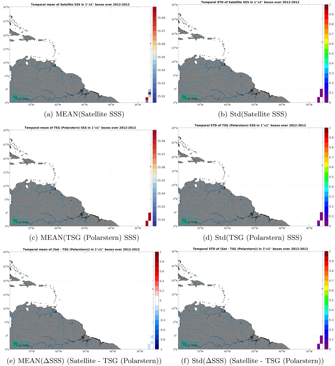
Figure 6: Temporal mean (left) and Std (right) of SSS from Aquarius SSS L3 OR v5 - 7-Day running - Rain mask (NASA-GSFC) (top), TSG (Polarstern) (middle), and of \Delta SSS (Satellite - TSG (Polarstern)). Only match-up pairs are used to generate these maps.
