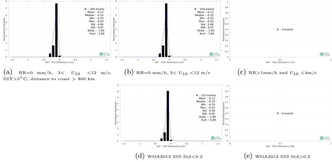
Figure 13: Normalized histogram of \Delta\text{SSS} (Aquarius SSS L3 OR v5 - 7-Day running - Rain mask (NASA-GSFC) - TSG (Polarstern)) for 5 different subdatasets corresponding to: RR=0 mm/h, 3 < U_{10} < 12 m/s, SST > 5^\circ\text{C} , distance to coast > 800 km (a), RR=0 mm/h, 3 < U_{10} < 12 m/s (b), RR > 1\text{mm/h} and U_{10} < 4\text{m/s} (c), WOA2013 SSS Std < 0.2 (d), WOA2013 SSS Std > 0.2 (e).
