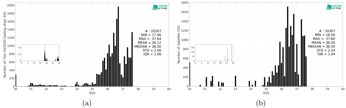
Figure 3: Histograms of SSS from TSG (GOSUD-Sailing-ship) (a) and Aquarius SSS L3 OR v5 - 7-Day running - Rain mask (NASA-GSFC) (b) considering all match-up pairs per bins of 0.1 over the Amazon and Orinoco river plumes Pi-MEP region and for the full satellite product period.
