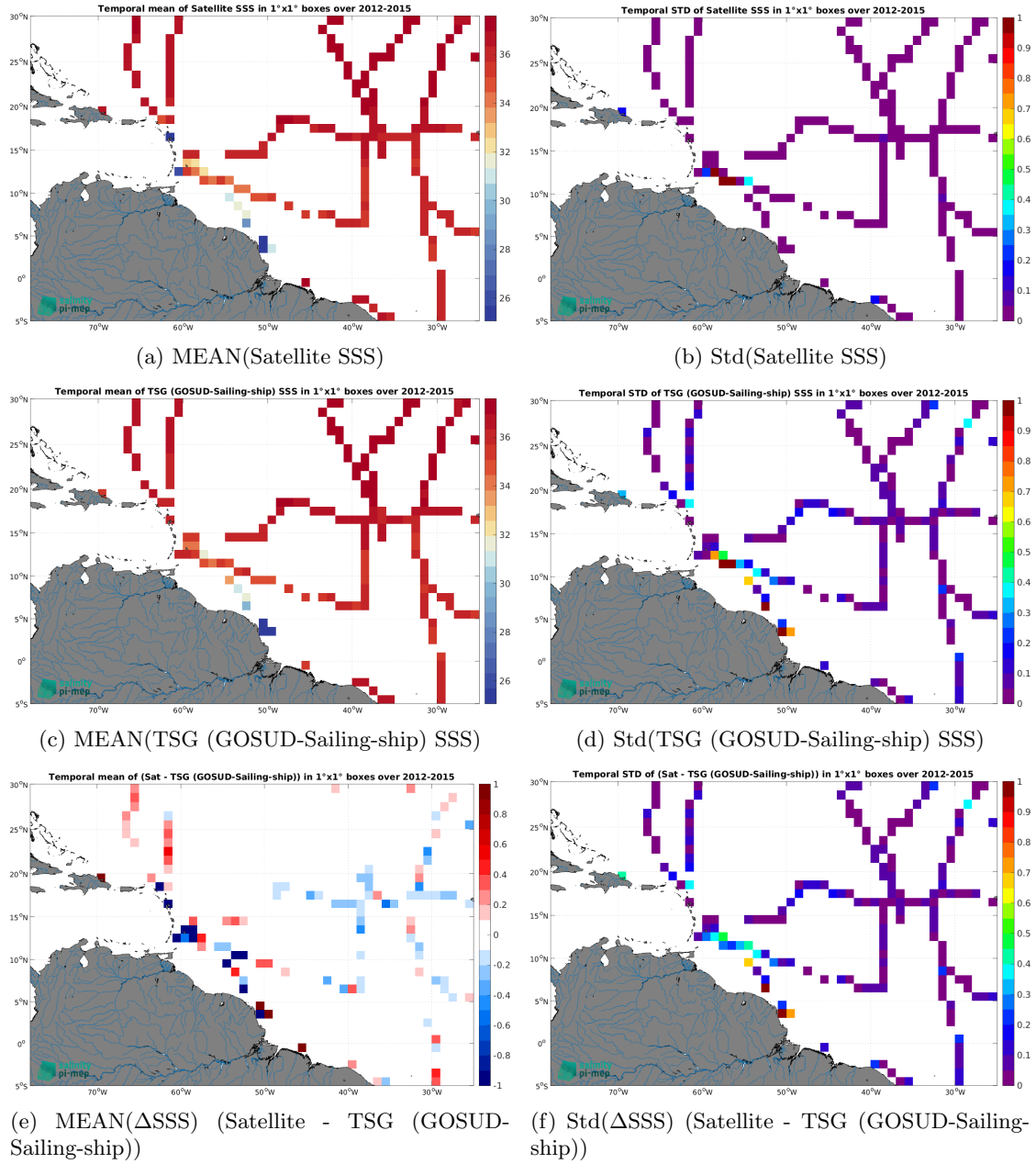
Figure 7: Temporal mean (left) and Std (right) of SSS from Aquarius SSS L3 OR v5 - 7-Day running - Rain mask (NASA-GSFC) (top), TSG (GOSUD-Sailing-ship) (middle), and of \Delta SSS (Satellite - TSG (GOSUD-Sailing-ship)). Only match-up pairs are used to generate these maps.
