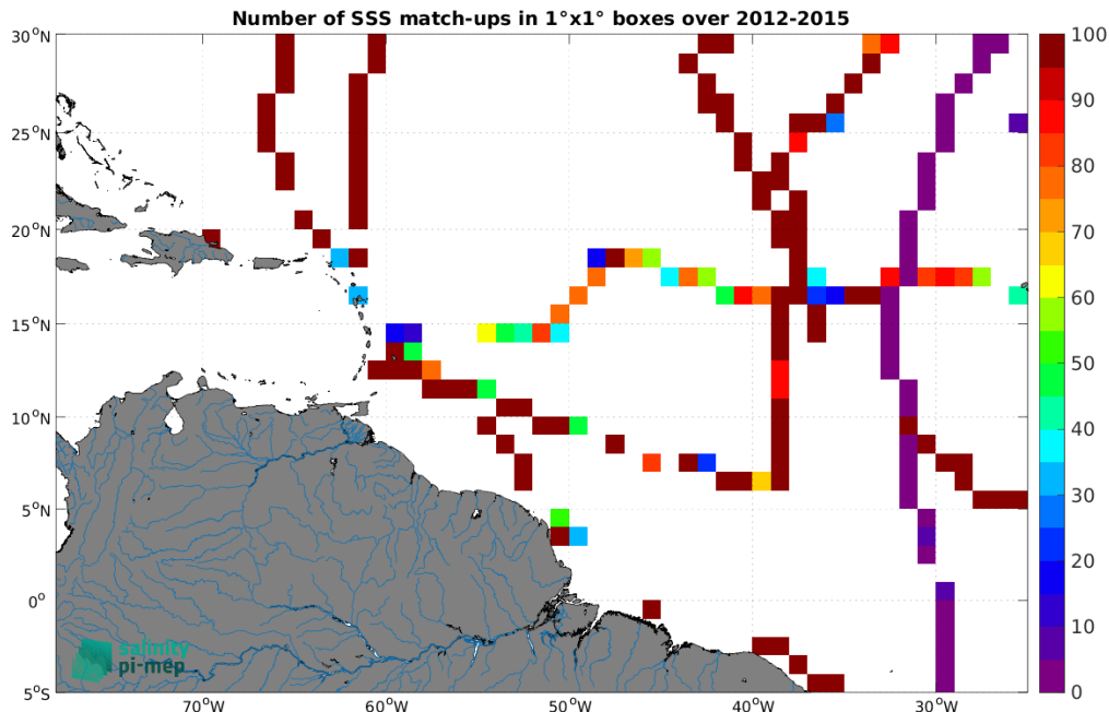
Figure 5: Number of SSS match-ups between TSG (GOSUD-Sailing-ship) SSS and the Aquarius SSS L3 OR v5 - 7-Day running - Rain mask (NASA-GSFC) SSS product for the Amazon and Orinoco river plumes Pi-MEP region over 1^\circ \times 1^\circ boxes and for the full satellite product period.
