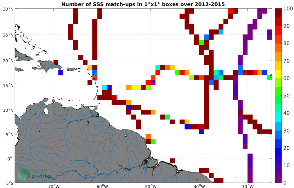
Figure 4: Number of SSS match-ups between TSG (GOSUD-Sailing-ship) SSS and the Aquarius SSS L3 OR v5 - 7-Day running - Rain mask (NASA-GSFC) SSS product for the Amazon and Orinoco river plumes Pi-MEP region over 1^\circ \times 1^\circ boxes and for the full satellite product period.
