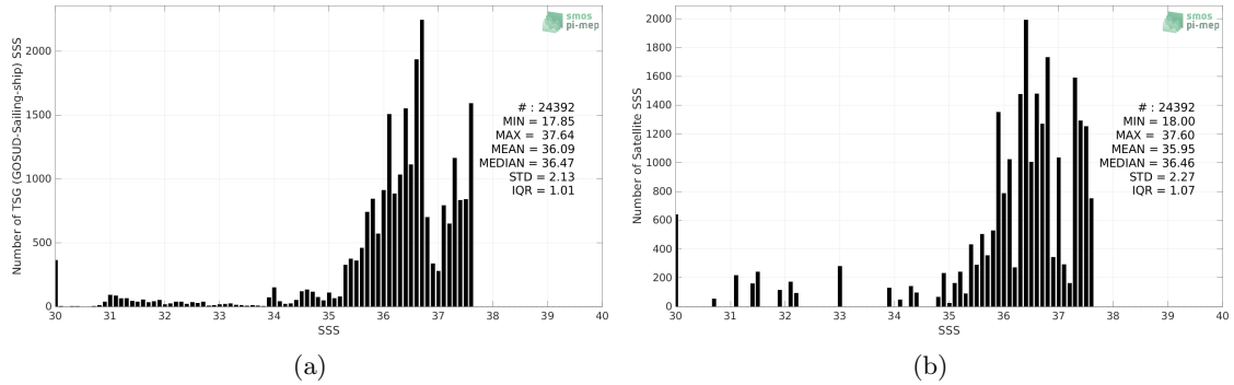
Figure 2: Histograms of SSS from TSG (GOSUD-Sailing-ship) (a) and Aquarius SSS L3 OR v5 - 7-Day running - Rain mask (NASA-GSFC) (b) considering all match-up pairs per bins of 0.1 over the Amazon and Orinoco river plumes Pi-MEP region and for the full satellite product period.
