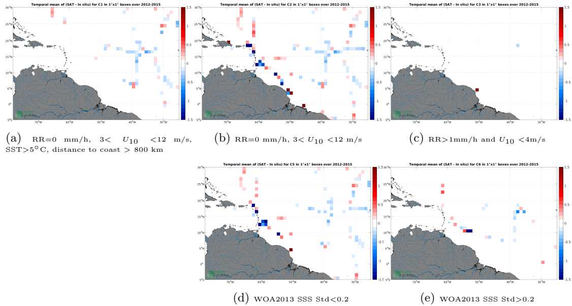
Figure 12: Temporal mean gridded over spatial boxes of size 1^{\circ}\times 1^{\circ} of \Delta SSS (Aquarius SSS L3 OR v5 - 7-Day running - Rain mask (NASA-GSFC) - TSG (GOSUD-Sailing-ship)) for 5 different subdatasets corresponding to:RR=0 mm/h, 3 < U_{10} < 12 m/s, SST >5^{\circ}\text{C} , distance to coast > 800 km (a), RR=0 mm/h, 3 < U_{10} < 12 m/s (b), RR >1 mm/h and U_{10} < 4 m/s (c), WOA2013 SSS Std <0.2 (d), WOA2013 SSS Std >0.2 (e).
