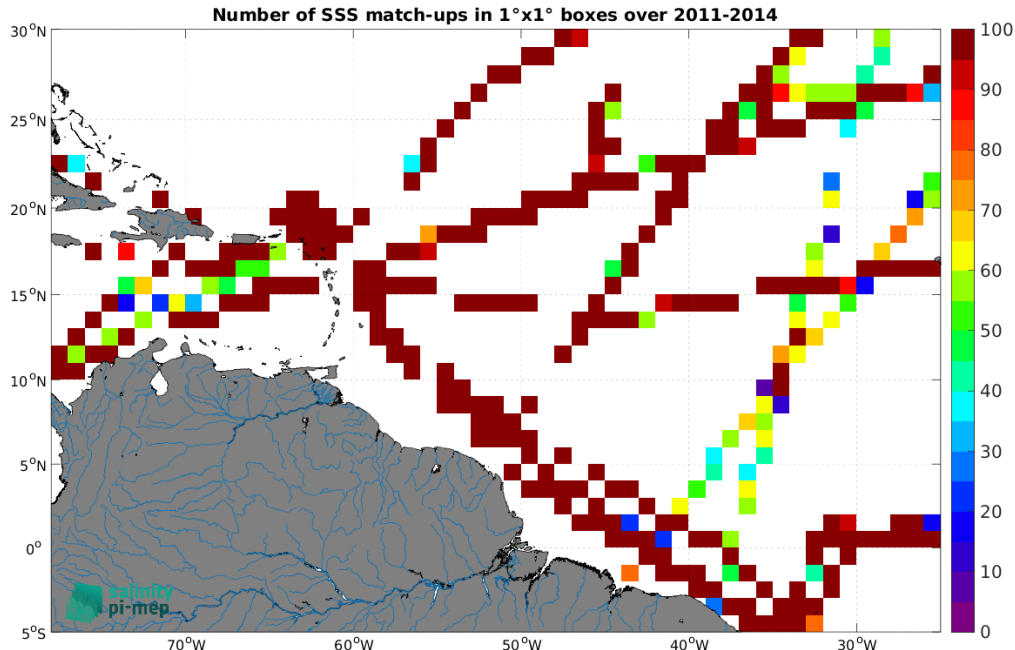
Figure 5: Number of SSS match-ups between TSG (GOSUD-Research-vessel) SSS and the Aquarius SSS L3 OR v5 - 7-Day running - Rain mask (NASA-GSFC) SSS product for the Amazon and Orinoco river plumes Pi-MEP region over 1^\circ \times 1^\circ boxes and for the full satellite product period.
