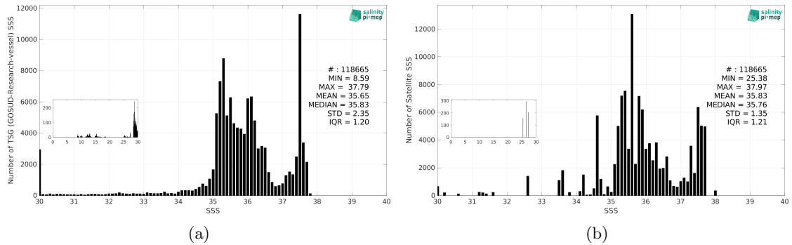
Figure 3: Histograms of SSS from TSG (GOSUD-Research-vessel) (a) and Aquarius SSS L3 OR v5 - 7-Day running - Rain mask (NASA-GSFC) (b) considering all match-up pairs per bins of 0.1 over the Amazon and Orinoco river plumes Pi-MEP region and for the full satellite product period.
