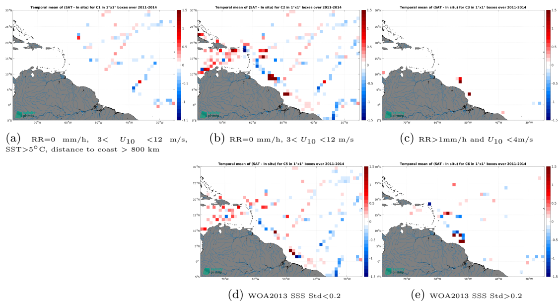
Figure 14: Temporal mean gridded over spatial boxes of size 1^\circ \times 1^\circ of \Delta SSS (Aquarius SSS L3 OR v5 - 7-Day running - Rain mask (NASA-GSFC) - TSG (GOSUD-Research-vessel)) for 5 different subdatasets corresponding to:RR=0 mm/h, 3 < U_{10} < 12 m/s, SST >5^\circ\text{C} , distance to coast > 800 km (a), RR=0 mm/h, 3 < U_{10} < 12 m/s (b), RR >1 mm/h and U_{10} < 4 m/s (c), WOA2013 SSS Std <0.2 (d), WOA2013 SSS Std >0.2 (e).
