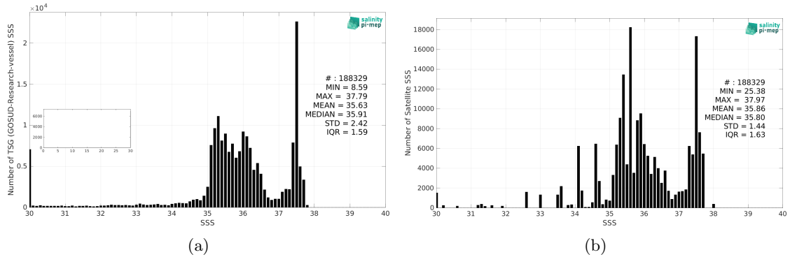
Figure 2: Histograms of SSS from TSG (GOSUD-Research-vessel) (a) and Aquarius SSS L3 OR v5 - 7-Day running - Rain mask (NASA-GSFC) (b) considering all match-up pairs per bins of 0.1 over the Amazon and Orinoco river plumes Pi-MEP region and for the full satellite product period.
