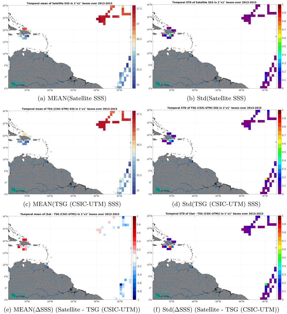
Figure 7: Temporal mean (left) and Std (right) of SSS from Aquarius SSS L3 OR v5 - 7-Day running - Rain mask (NASA-GSFC) (top), TSG (CSIC-UTM) (middle), and of \Delta SSS (Satellite - TSG (CSIC-UTM)). Only match-up pairs are used to generate these maps.
