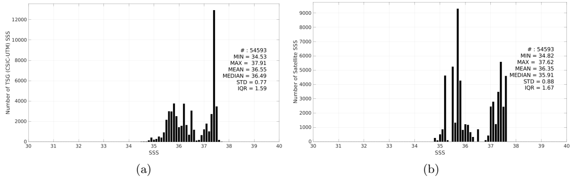
Figure 3: Histograms of SSS from TSG (CSIC-UTM) (a) and Aquarius SSS L3 OR v5 - 7-Day running - Rain mask (NASA-GSFC) (b) considering all match-up pairs per bins of 0.1 over the Amazon and Orinoco river plumes Pi-MEP region and for the full satellite product period.
