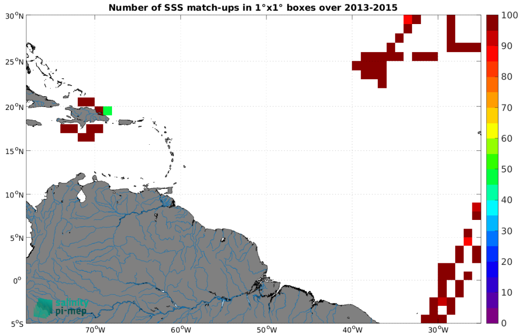
Figure 5: Number of SSS match-ups between TSG (CSIC-UTM) SSS and the Aquarius SSS L3 OR v5 - 7-Day running - Rain mask (NASA-GSFC) SSS product for the Amazon and Orinoco river plumes Pi-MEP region over 1^\circ \times 1^\circ boxes and for the full satellite product period.
