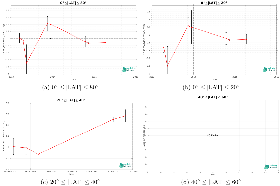
Figure 10: Monthly median (red curves) of \Delta SSS (Satellite - in situ ) between Aquarius SSS L3 OR v5 - 7-Day running - Rain mask (NASA-GSFC) and TSG (CSIC-UTM) SSS as function of time for all the collected Pi-MEP match-up pairs estimated over the Amazon and Orinoco river plumes Pi-MEP region and for the full satellite product period are shown for different latitude bands: (a) 80^\circ\text{S}-80^\circ\text{N} , (b) 20^\circ\text{S}-20^\circ\text{N} , (c) 40^\circ\text{S}-20^\circ\text{S} and 20^\circ\text{N}-40^\circ\text{N} and (d) 60^\circ\text{S}-40^\circ\text{S} and 40^\circ\text{N}-60^\circ\text{N} .
