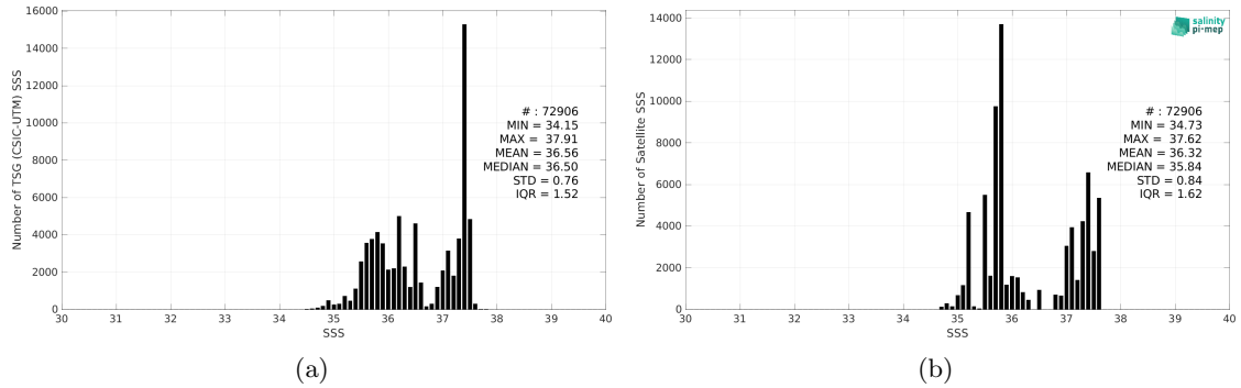
Figure 2: Histograms of SSS from TSG (CSIC-UTM) (a) and Aquarius SSS L3 OR v5 - 7-Day running - Rain mask (NASA-GSFC) (b) considering all match-up pairs per bins of 0.1 over the Amazon and Orinoco river plumes Pi-MEP region and for the full satellite product period.
