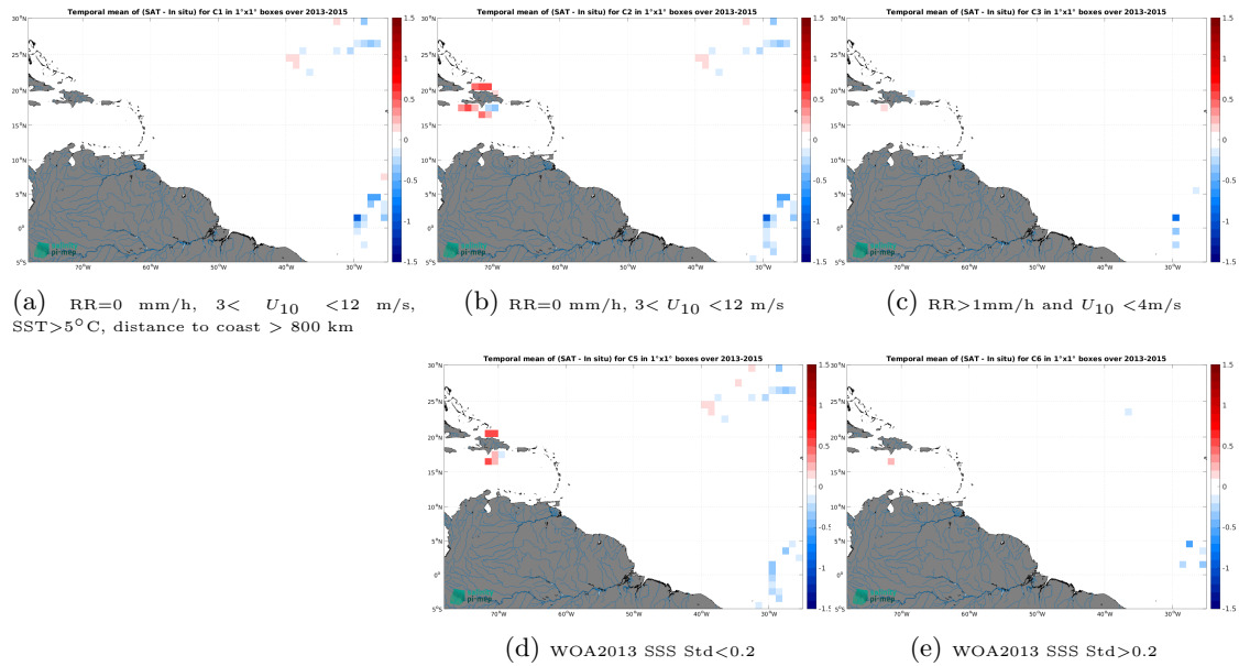
Figure 12: Temporal mean gridded over spatial boxes of size 1^{\circ}\times 1^{\circ} of \Delta\text{SSS} (Aquarius SSS L3 OR v5 - 7-Day running - Rain mask (NASA-GSFC) - TSG (CSIC-UTM)) for 5 different subdatasets corresponding to:RR=0 mm/h, 3 < U_{10} < 12 m/s, SST >5^{\circ}\text{C} , distance to coast > 800 km (a), RR=0 mm/h, 3 < U_{10} < 12 m/s (b), RR >1 mm/h and U_{10} < 4 m/s (c), WOA2013 SSS Std <0.2 (d), WOA2013 SSS Std >0.2 (e).
