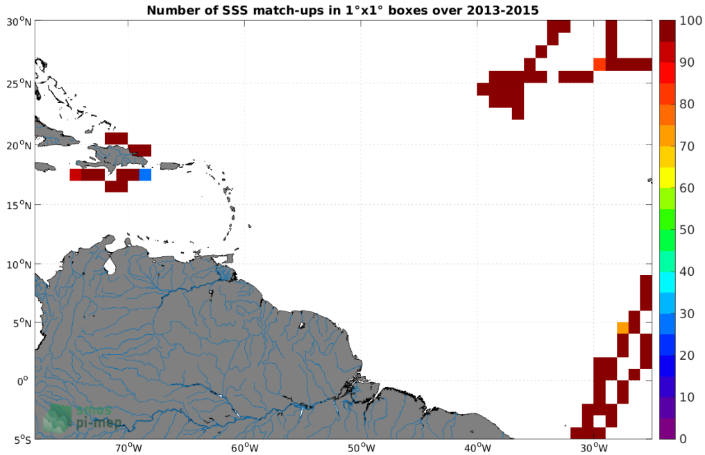
Figure 4: Number of SSS match-ups between TSG (CSIC-UTM) SSS and the Aquarius SSS L3 OR v5 - 7-Day running - Rain mask (NASA-GSFC) SSS product for the Amazon and Orinoco river plumes Pi-MEP region over 1^\circ \times 1^\circ boxes and for the full satellite product period.
