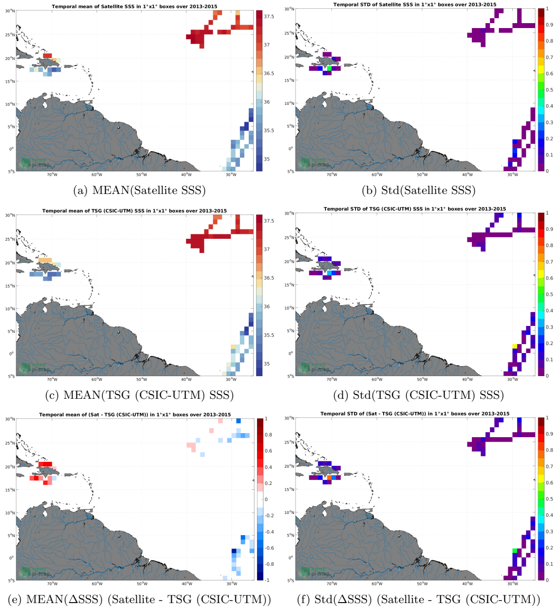
Figure 6: Temporal mean (left) and Std (right) of SSS from Aquarius SSS L3 OR v5 - 7-Day running - Rain mask (NASA-GSFC) (top), TSG (CSIC-UTM) (middle), and of \Delta SSS (Satellite - TSG (CSIC-UTM)). Only match-up pairs are used to generate these maps.
