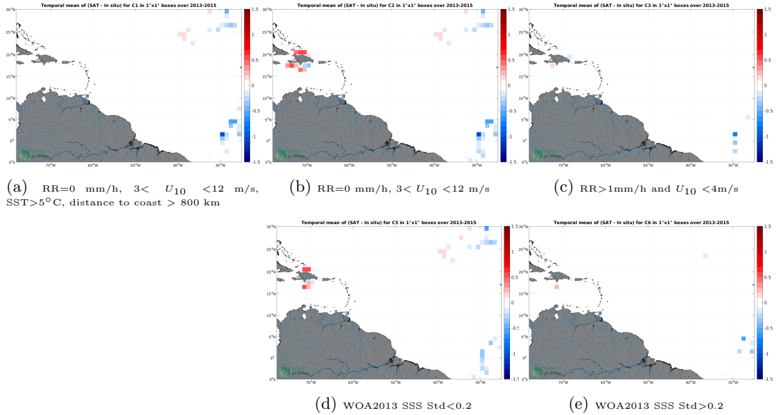
Figure 12: Temporal mean gridded over spatial boxes of size 1^{\circ}\times 1^{\circ} of \Delta\text{SSS} (Aquarius SSS L3 OR v5 - 7-Day running - Rain mask (NASA-GSFC) - TSG (CSIC-UTM)) for 5 different subdatasets corresponding to:RR=0 mm/h, 3 < U_{10} < 12 m/s, SST >5^{\circ}\text{C} , distance to coast > 800 km (a), RR=0 mm/h, 3 < U_{10} < 12 m/s (b), RR >1 mm/h and U_{10} < 4 m/s (c), WOA2013 SSS Std <0.2 (d), WOA2013 SSS Std >0.2 (e).
