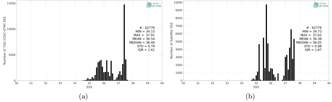
Figure 2: Histograms of SSS from TSG (CSIC-UTM) (a) and Aquarius SSS L3 OR v5 - 7-Day running - Rain mask (NASA-GSFC) (b) considering all match-up pairs per bins of 0.1 over the Amazon and Orinoco river plumes Pi-MEP region and for the full satellite product period.
