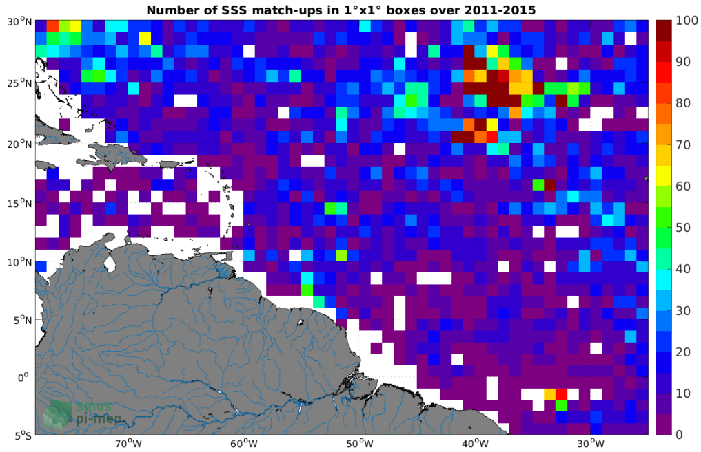
Figure 4: Number of SSS match-ups between Argo SSS and the Aquarius SSS L3 OR v5 - 7-Day running - Rain mask (NASA-GSFC) SSS product for the Amazon and Orinoco river plumes Pi-MEP region over 1^\circ \times 1^\circ boxes and for the full satellite product period.
