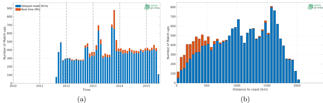
Figure 1: Number of match-ups between Argo and Aquarius SSS L3 OR v5 - 7-Day running - Rain mask (NASA-GSFC) SSS as a function of time (a) and as function of the distance to coast (b) over the Amazon and Orinoco river plumes Pi-MEP region and for the full satellite product period.
