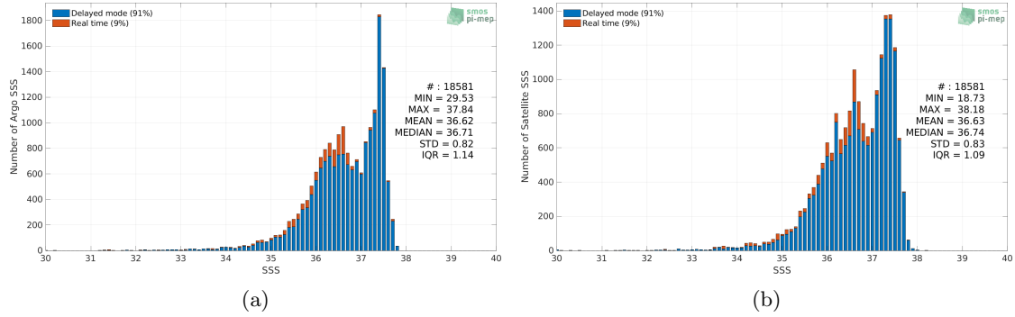
Figure 2: Histograms of SSS from Argo (a) and Aquarius SSS L3 OR v5 - 7-Day running - Rain mask (NASA-GSFC) (b) considering all match-up pairs per bins of 0.1 over the Amazon and Orinoco river plumes Pi-MEP region and for the full satellite product period.
