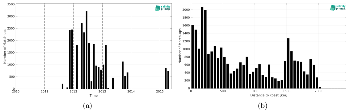
Figure 2: Number of match-ups between TSG (SAMOS) and Aquarius SSS L3 OR v5 - Monthly (NASA-GSFC) SSS as a function of time (a) and as function of the distance to coast (b) over the Amazon and Orinoco river plumes Pi-MEP region and for the full satellite product period.
