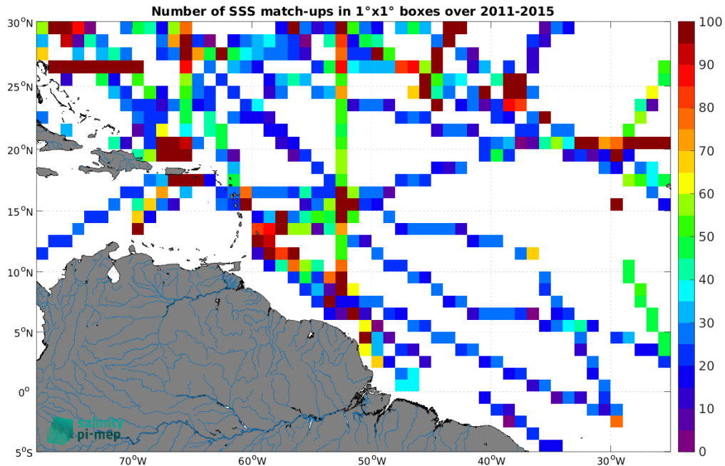
Figure 5: Number of SSS match-ups between TSG (SAMOS) SSS and the Aquarius SSS L3 OR v5 - Monthly (NASA-GSFC) SSS product for the Amazon and Orinoco river plumes Pi-MEP region over 1^\circ \times 1^\circ boxes and for the full satellite product period.
