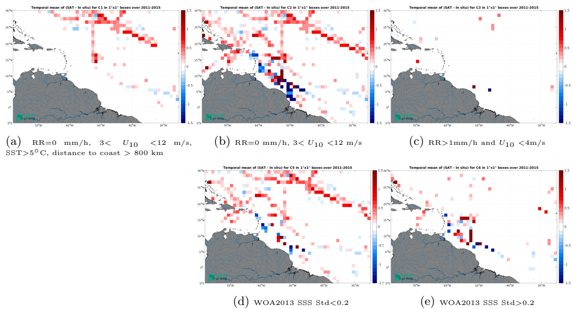
Figure 14: Temporal mean gridded over spatial boxes of size 1^\circ \times 1^\circ of \Delta\text{SSS} (Aquarius SSS L3 OR v5 - Monthly (NASA-GSFC) - TSG (SAMOS)) for 5 different subdatasets corresponding to:RR=0 mm/h, 3 < U_{10} < 12 m/s, SST >5^\circ\text{C} , distance to coast > 800 km (a), RR=0 mm/h, 3 < U_{10} < 12 m/s (b), RR >1 mm/h and U_{10} < 4 m/s (c), WOA2013 SSS Std <0.2 (d), WOA2013 SSS Std >0.2 (e).
