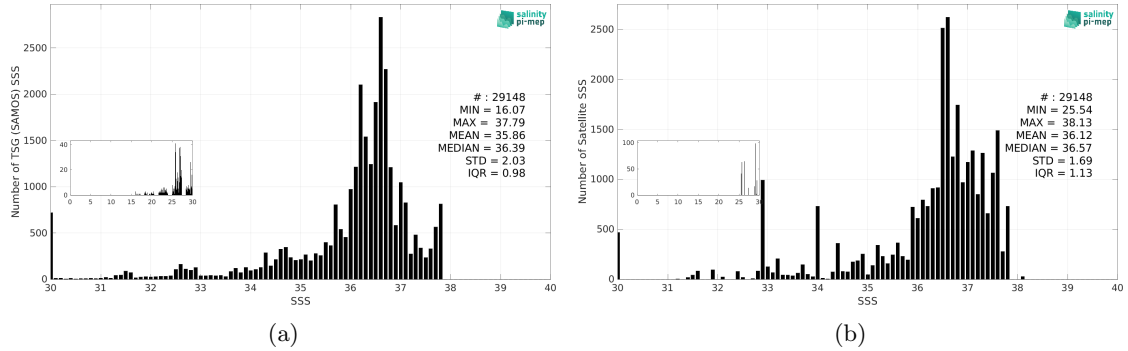
Figure 3: Histograms of SSS from TSG (SAMOS) (a) and Aquarius SSS L3 OR v5 - Monthly (NASA-GSFC) (b) considering all match-up pairs per bins of 0.1 over the Amazon and Orinoco river plumes Pi-MEP region and for the full satellite product period.
