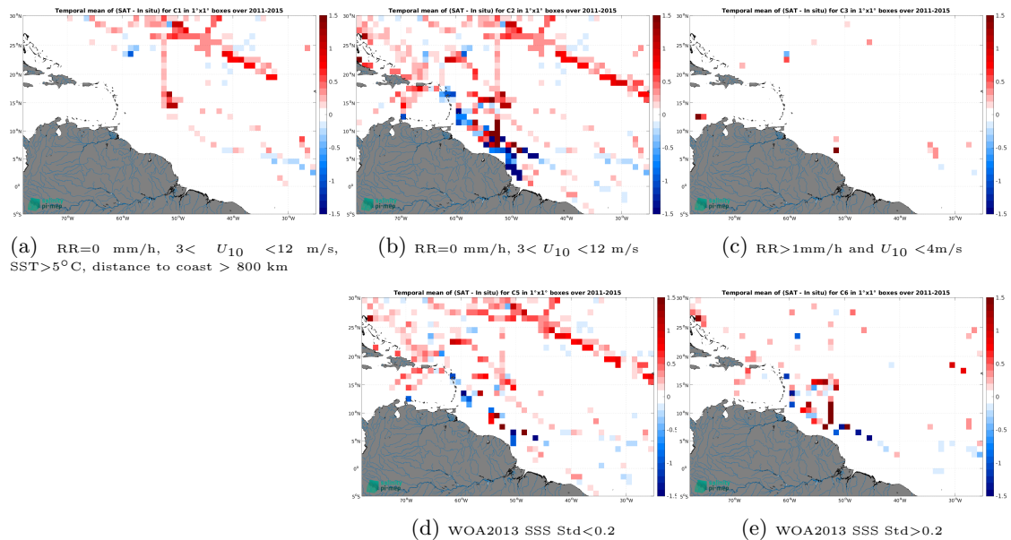
Figure 12: Temporal mean gridded over spatial boxes of size 1^\circ \times 1^\circ of \Delta\text{SSS} (Aquarius SSS L3 OR v5 - Monthly (NASA-GSFC) - TSG (SAMOS)) for 5 different subdatasets corresponding to:RR=0 mm/h, 3 < U_{10} < 12 m/s, SST >5^\circ\text{C} , distance to coast > 800 km (a), RR=0 mm/h, 3 < U_{10} < 12 m/s (b), RR >1 mm/h and U_{10} < 4 m/s (c), WOA2013 SSS Std <0.2 (d), WOA2013 SSS Std >0.2 (e).
