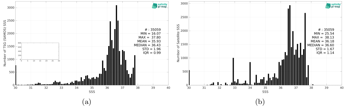
Figure 2: Histograms of SSS from TSG (SAMOS) (a) and Aquarius SSS L3 OR v5 - Monthly (NASA-GSFC) (b) considering all match-up pairs per bins of 0.1 over the Amazon and Orinoco river plumes Pi-MEP region and for the full satellite product period.
