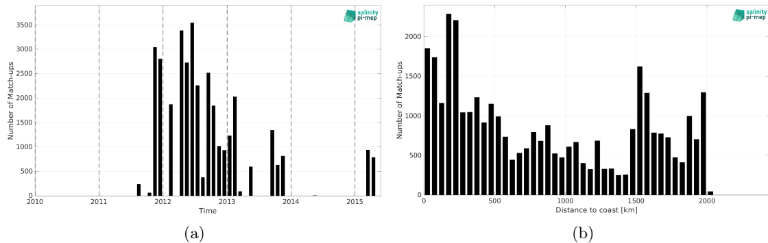
Figure 1: Number of match-ups between TSG (SAMOS) and Aquarius SSS L3 OR v5 - Monthly (NASA-GSFC) SSS as a function of time (a) and as function of the distance to coast (b) over the Amazon and Orinoco river plumes Pi-MEP region and for the full satellite product period.
