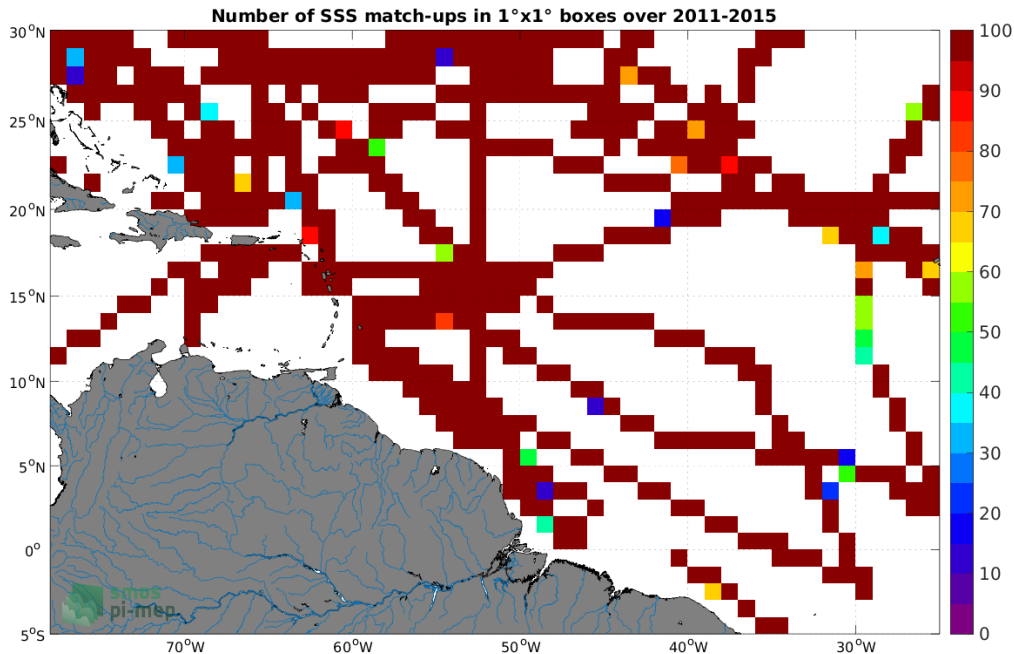
Figure 4: Number of SSS match-ups between TSG (SAMOS) SSS and the Aquarius SSS L3 OR v5 - Monthly (NASA-GSFC) SSS product for the Amazon and Orinoco river plumes Pi-MEP region over 1^\circ \times 1^\circ boxes and for the full satellite product period.
