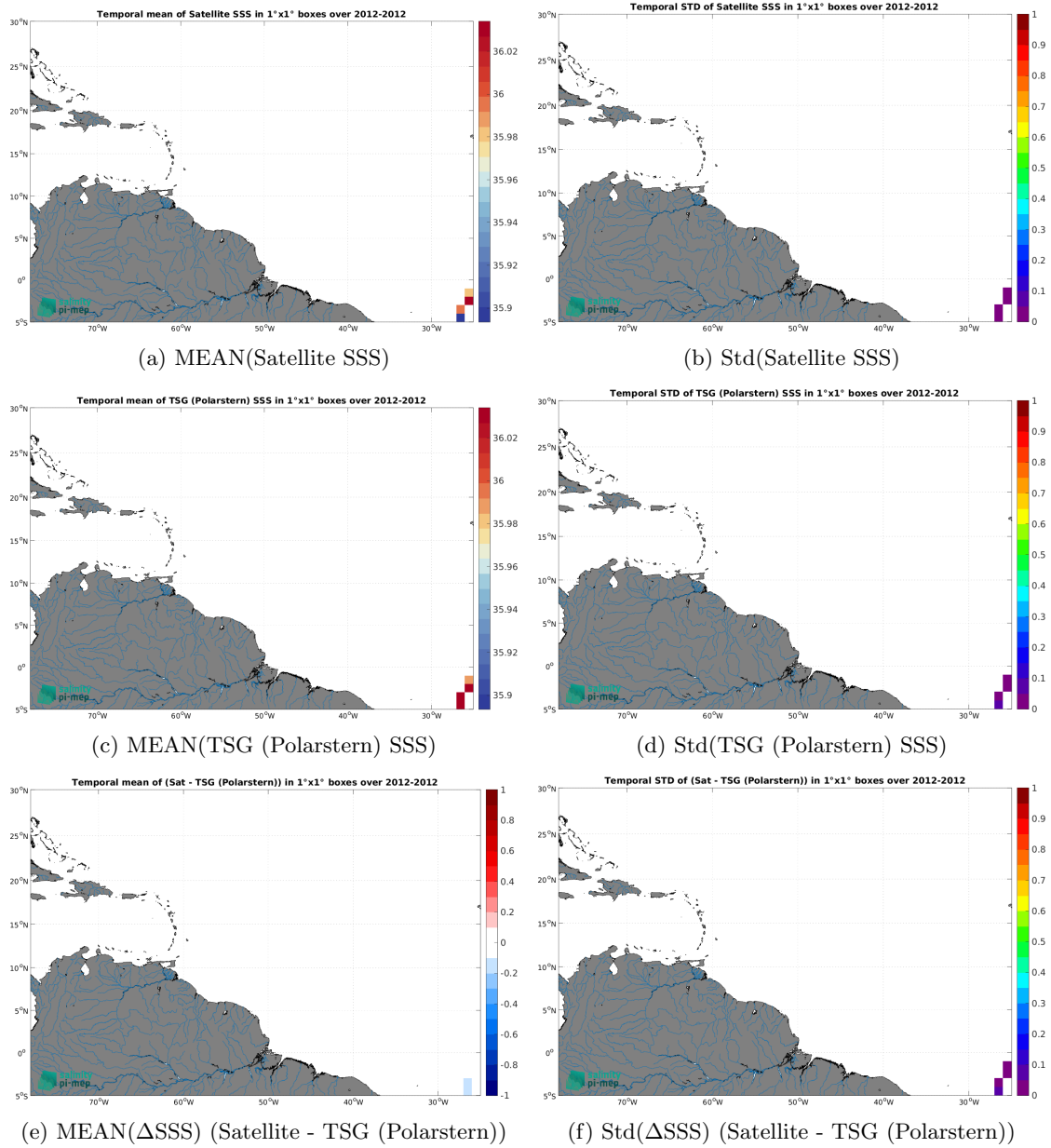
Figure 7: Temporal mean (left) and Std (right) of SSS from Aquarius SSS L3 OR v5 - Monthly (NASA-GSFC) (top), TSG (Polarstern) (middle), and of \Delta SSS (Satellite - TSG (Polarstern)). Only match-up pairs are used to generate these maps.
