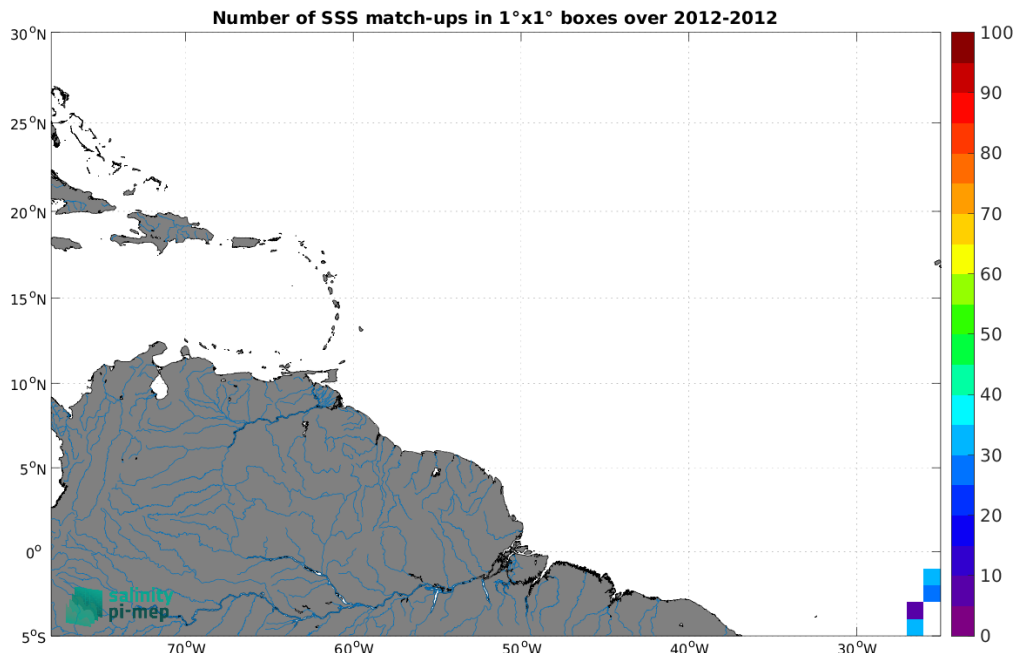
Figure 5: Number of SSS match-ups between TSG (Polarstern) SSS and the Aquarius SSS L3 OR v5 - Monthly (NASA-GSFC) SSS product for the Amazon and Orinoco river plumes Pi-MEP region over 1^\circ \times 1^\circ boxes and for the full satellite product period.
