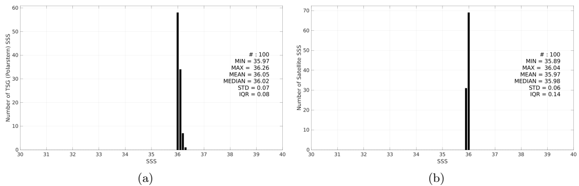
Figure 3: Histograms of SSS from TSG (Polarstern) (a) and Aquarius SSS L3 OR v5 - Monthly (NASA-GSFC) (b) considering all match-up pairs per bins of 0.1 over the Amazon and Orinoco river plumes Pi-MEP region and for the full satellite product period.
