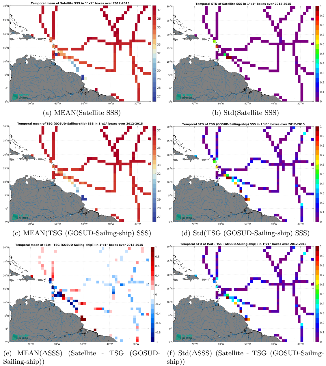
Figure 7: Temporal mean (left) and Std (right) of SSS from Aquarius SSS L3 OR v5 - Monthly (NASA-GSFC) (top), TSG (GOSUD-Sailing-ship) (middle), and of \Delta SSS (Satellite - TSG (GOSUD-Sailing-ship)). Only match-up pairs are used to generate these maps.
