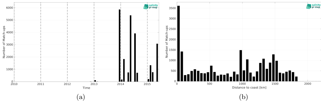
Figure 2: Number of match-ups between TSG (GOSUD-Sailing-ship) and Aquarius SSS L3 OR v5 - Monthly (NASA-GSFC) SSS as a function of time (a) and as function of the distance to coast (b) over the Amazon and Orinoco river plumes Pi-MEP region and for the full satellite product period.
