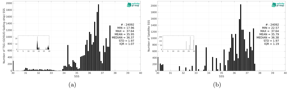
Figure 3: Histograms of SSS from TSG (GOSUD-Sailing-ship) (a) and Aquarius SSS L3 OR v5 - Monthly (NASA-GSFC) (b) considering all match-up pairs per bins of 0.1 over the Amazon and Orinoco river plumes Pi-MEP region and for the full satellite product period.
