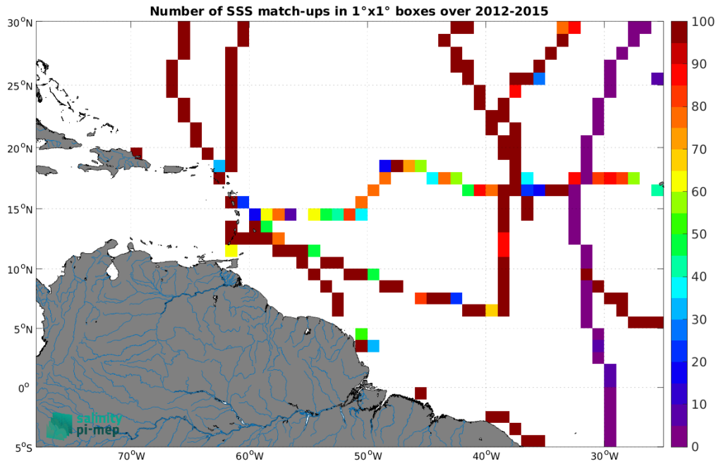
Figure 5: Number of SSS match-ups between TSG (GOSUD-Sailing-ship) SSS and the Aquarius SSS L3 OR v5 - Monthly (NASA-GSFC) SSS product for the Amazon and Orinoco river plumes Pi-MEP region over 1^\circ \times 1^\circ boxes and for the full satellite product period.
