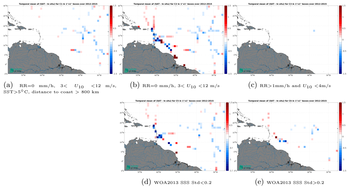
Figure 14: Temporal mean gridded over spatial boxes of size 1^\circ \times 1^\circ of \Delta SSS (Aquarius SSS L3 OR v5 - Monthly (NASA-GSFC) - TSG (GOSUD-Sailing-ship)) for 5 different subdatasets corresponding to:RR=0 mm/h, 3 < U_{10} < 12 m/s, SST >5^\circ\text{C} , distance to coast > 800 km (a), RR=0 mm/h, 3 < U_{10} < 12 m/s (b), RR >1 mm/h and U_{10} < 4 m/s (c), WOA2013 SSS Std <0.2 (d), WOA2013 SSS Std >0.2 (e).
