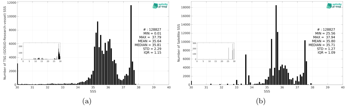
Figure 3: Histograms of SSS from TSG (GOSUD-Research-vessel) (a) and Aquarius SSS L3 OR v5 - Monthly (NASA-GSFC) (b) considering all match-up pairs per bins of 0.1 over the Amazon and Orinoco river plumes Pi-MEP region and for the full satellite product period.
