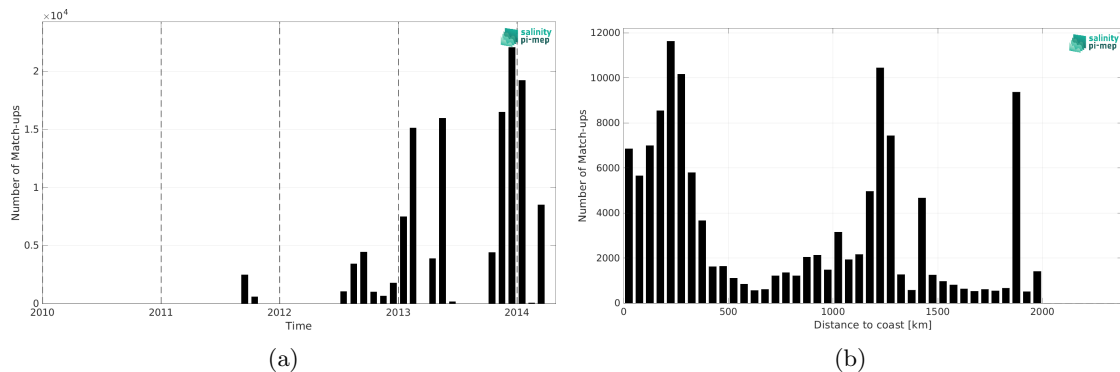
Figure 2: Number of match-ups between TSG (GOSUD-Research-vessel) and Aquarius SSS L3 OR v5 - Monthly (NASA-GSFC) SSS as a function of time (a) and as function of the distance to coast (b) over the Amazon and Orinoco river plumes Pi-MEP region and for the full satellite product period.
