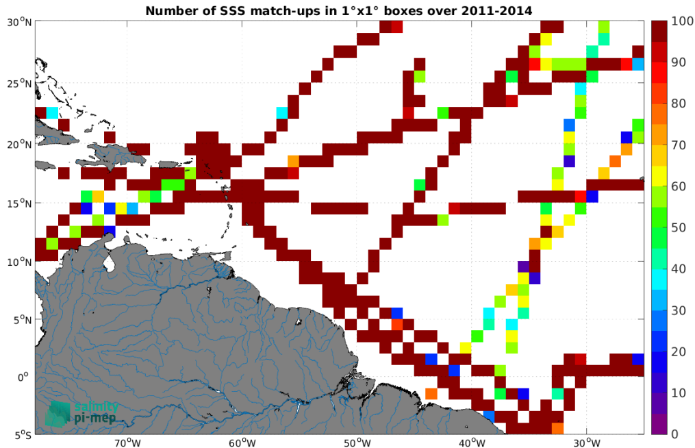
Figure 5: Number of SSS match-ups between TSG (GOSUD-Research-vessel) SSS and the Aquarius SSS L3 OR v5 - Monthly (NASA-GSFC) SSS product for the Amazon and Orinoco river plumes Pi-MEP region over 1^\circ \times 1^\circ boxes and for the full satellite product period.
