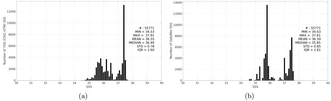
Figure 3: Histograms of SSS from TSG (CSIC-UTM) (a) and Aquarius SSS L3 OR v5 - Monthly (NASA-GSFC) (b) considering all match-up pairs per bins of 0.1 over the Amazon and Orinoco river plumes Pi-MEP region and for the full satellite product period.
