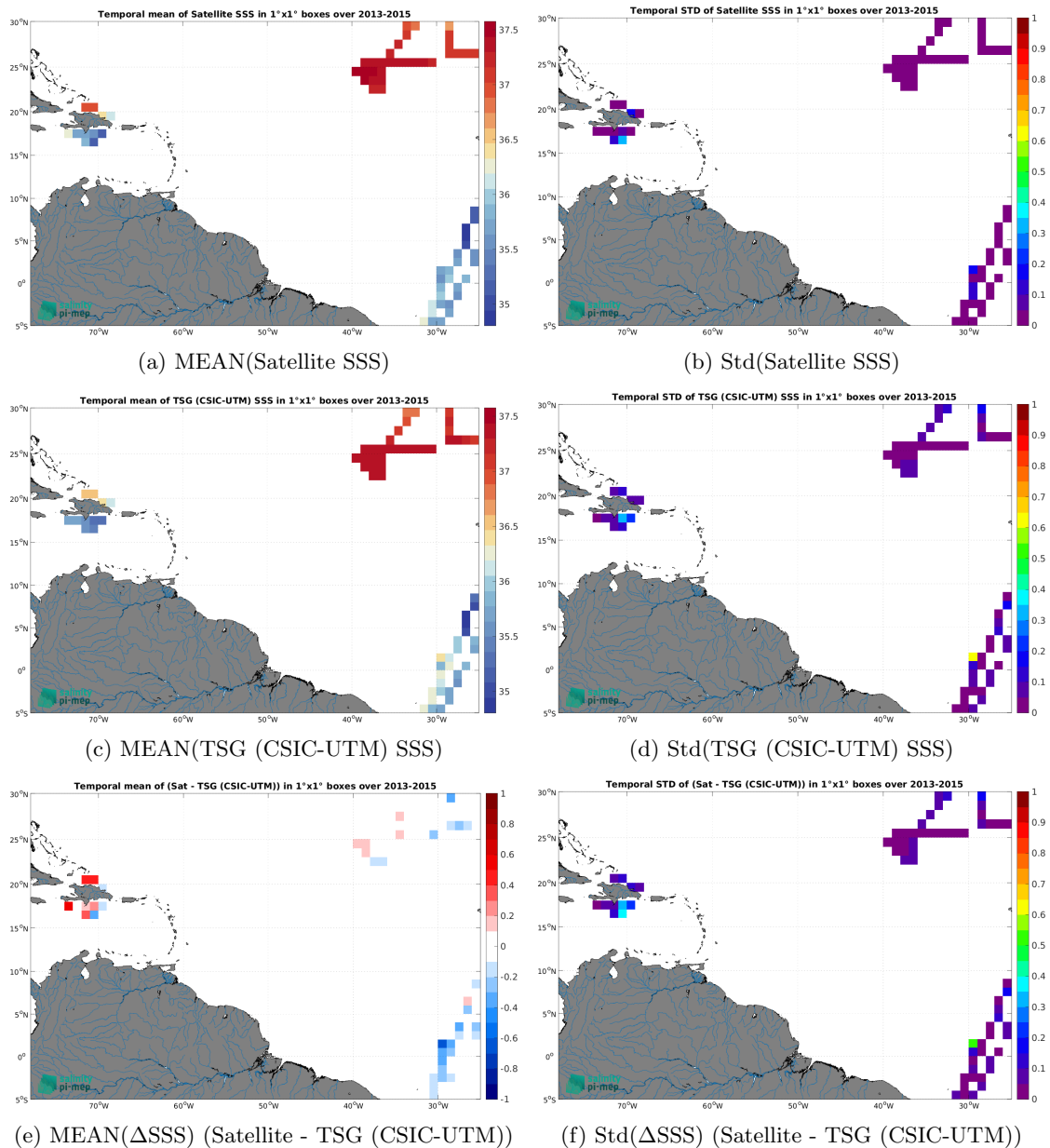
Figure 7: Temporal mean (left) and Std (right) of SSS from Aquarius SSS L3 OR v5 - Monthly (NASA-GSFC) (top), TSG (CSIC-UTM) (middle), and of \Delta SSS (Satellite - TSG (CSIC-UTM)). Only match-up pairs are used to generate these maps.
