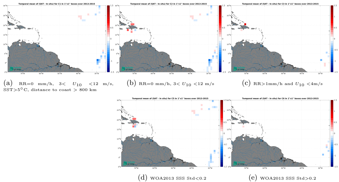
Figure 14: Temporal mean gridded over spatial boxes of size 1^\circ \times 1^\circ of \Delta SSS (Aquarius SSS L3 OR v5 - Monthly (NASA-GSFC) - TSG (CSIC-UTM)) for 5 different subdatasets corresponding to:RR=0 mm/h, 3 < U_{10} < 12 m/s, SST >5^\circ C, distance to coast > 800 km (a), RR=0 mm/h, 3 < U_{10} < 12 m/s (b), RR >1 mm/h and U_{10} < 4 m/s (c), WOA2013 SSS Std <0.2 (d), WOA2013 SSS Std >0.2 (e).
