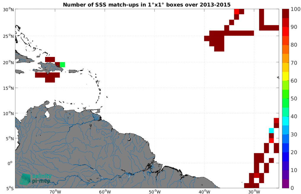
Figure 5: Number of SSS match-ups between TSG (CSIC-UTM) SSS and the Aquarius SSS L3 OR v5 - Monthly (NASA-GSFC) SSS product for the Amazon and Orinoco river plumes Pi-MEP region over 1^\circ \times 1^\circ boxes and for the full satellite product period.
