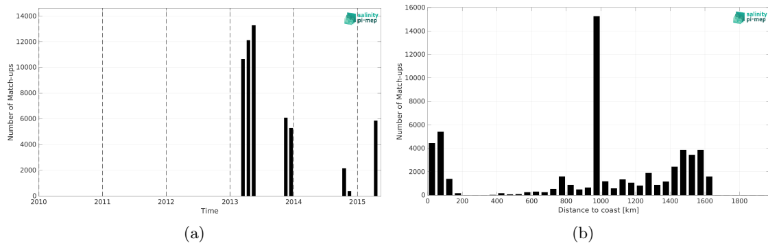
Figure 2: Number of match-ups between TSG (CSIC-UTM) and Aquarius SSS L3 OR v5 - Monthly (NASA-GSFC) SSS as a function of time (a) and as function of the distance to coast (b) over the Amazon and Orinoco river plumes Pi-MEP region and for the full satellite product period.
