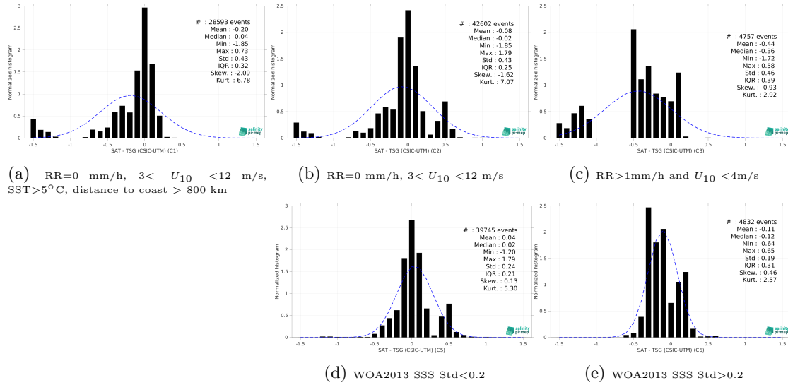
Figure 13: Normalized histogram of \Delta\text{SSS} (Aquarius SSS L3 OR v5 - Monthly (NASA-GSFC) - TSG (CSIC-UTM)) for 5 different subdatasets corresponding to: RR=0 mm/h, 3 < U_{10} < 12 m/s, SST>5°C, distance to coast > 800 km (a), RR=0 mm/h, 3 < U_{10} < 12 m/s (b), RR>1mm/h and U_{10} < 4 m/s (c), WOA2013 SSS Std<0.2 (d), WOA2013 SSS Std>0.2 (e).
