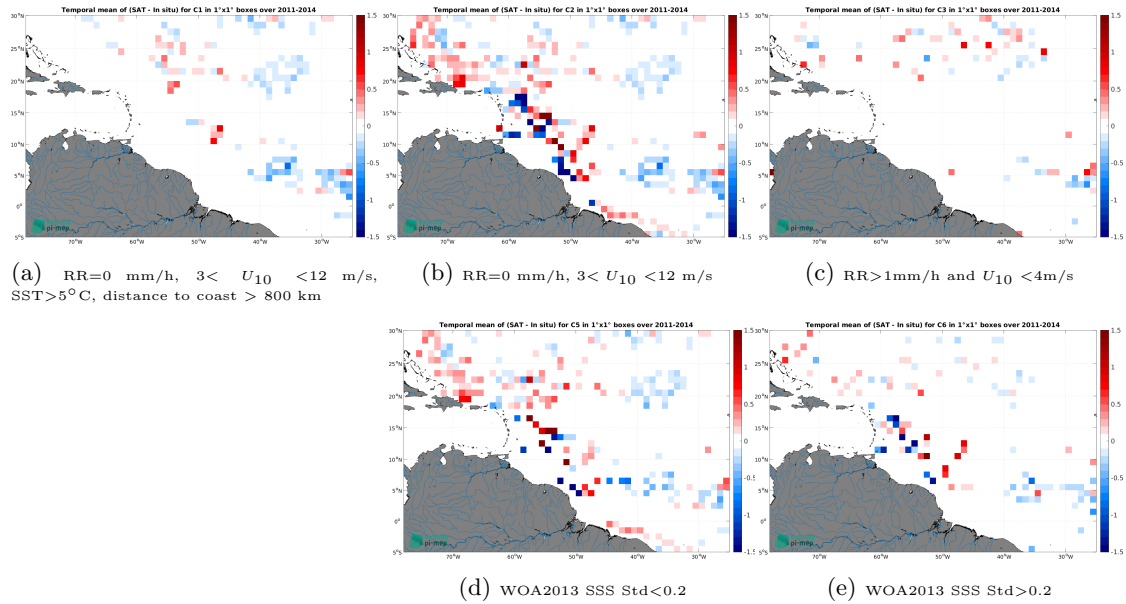
Figure 11: Temporal mean gridded over spatial boxes of size 1^\circ \times 1^\circ of \Delta\text{SSS} (Aquarius SSS L3 OR v5 - Monthly (NASA-GSFC) - Surface drifters) for 5 different subdatasets corresponding to:RR=0 mm/h, 3 < U_{10} < 12 m/s, SST >5^\circ\text{C} , distance to coast > 800 km (a), RR=0 mm/h, 3 < U_{10} < 12 m/s (b), RR >1 mm/h and U_{10} < 4 m/s (c), WOA2013 SSS Std <0.2 (d), WOA2013 SSS Std >0.2 (e).
