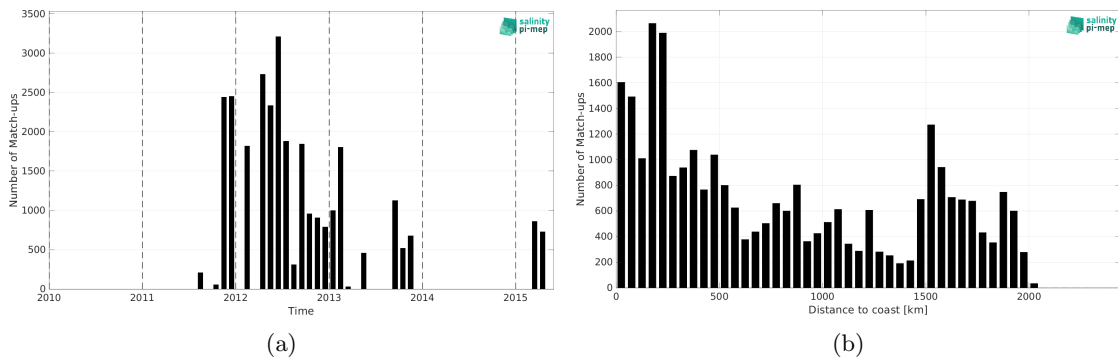
Figure 2: Number of match-ups between TSG (SAMOS) and Aquarius SSS L3 OR v5 - Monthly - Rain mask (NASA-GSFC) SSS as a function of time (a) and as function of the distance to coast (b) over the Amazon and Orinoco river plumes Pi-MEP region and for the full satellite product period.
