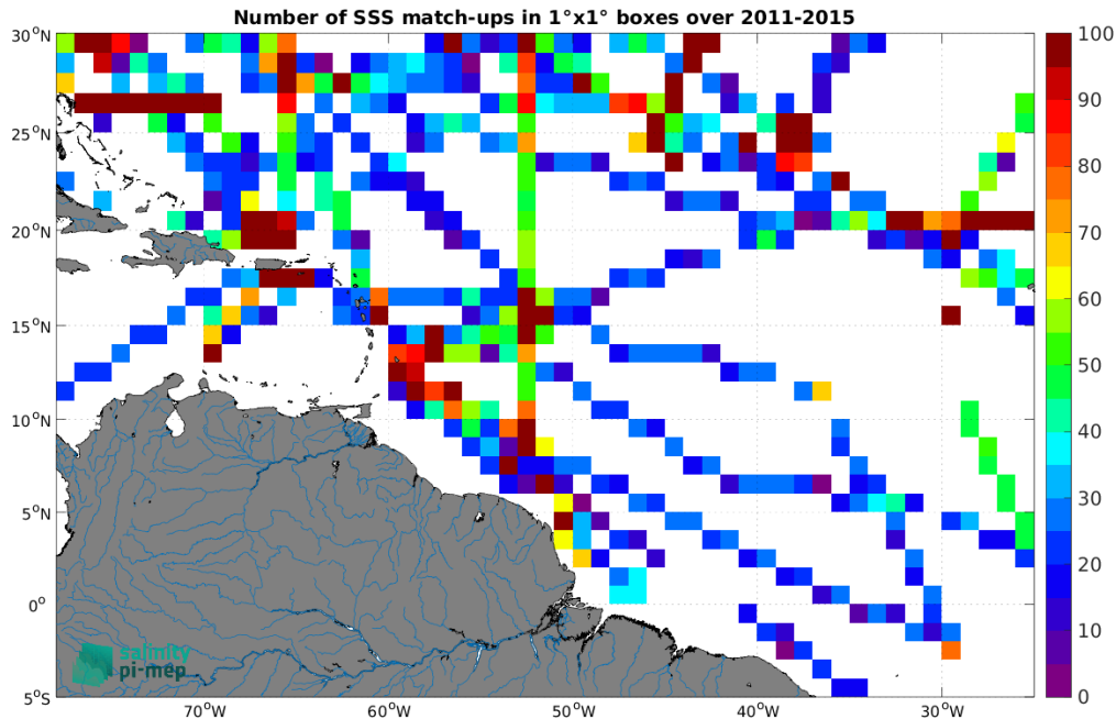
Figure 5: Number of SSS match-ups between TSG (SAMOS) SSS and the Aquarius SSS L3 OR v5 - Monthly - Rain mask (NASA-GSFC) SSS product for the Amazon and Orinoco river plumes Pi-MEP region over 1^\circ \times 1^\circ boxes and for the full satellite product period.
