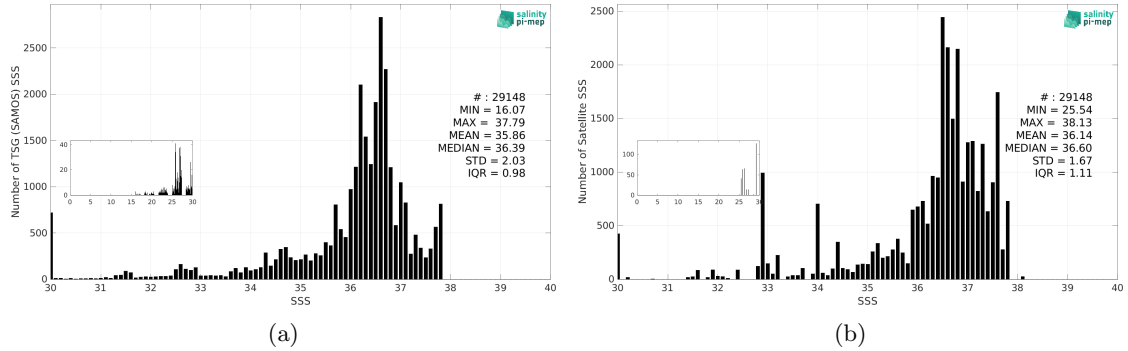
Figure 3: Histograms of SSS from TSG (SAMOS) (a) and Aquarius SSS L3 OR v5 - Monthly - Rain mask (NASA-GSFC) (b) considering all match-up pairs per bins of 0.1 over the Amazon and Orinoco river plumes Pi-MEP region and for the full satellite product period.
