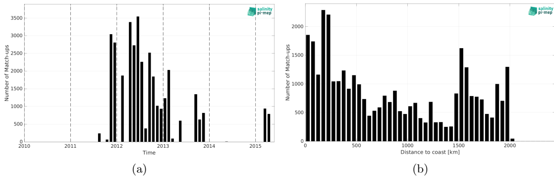
Figure 1: Number of match-ups between TSG (SAMOS) and Aquarius SSS L3 OR v5 - Monthly - Rain mask (NASA-GSFC) SSS as a function of time (a) and as function of the distance to coast (b) over the Amazon and Orinoco river plumes Pi-MEP region and for the full satellite product period.
