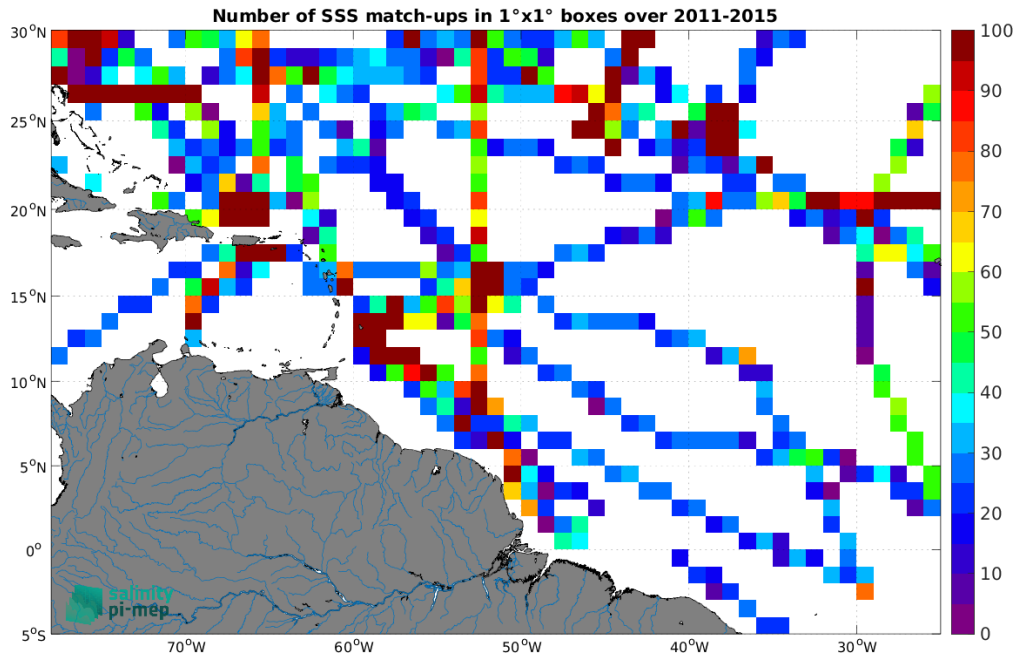
Figure 4: Number of SSS match-ups between TSG (SAMOS) SSS and the Aquarius SSS L3 OR v5 - Monthly - Rain mask (NASA-GSFC) SSS product for the Amazon and Orinoco river plumes Pi-MEP region over 1^\circ \times 1^\circ boxes and for the full satellite product period.
