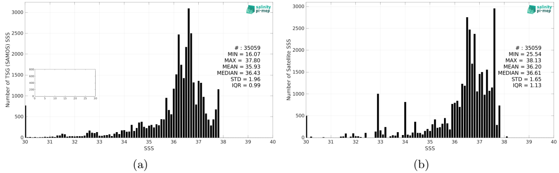
Figure 2: Histograms of SSS from TSG (SAMOS) (a) and Aquarius SSS L3 OR v5 - Monthly - Rain mask (NASA-GSFC) (b) considering all match-up pairs per bins of 0.1 over the Amazon and Orinoco river plumes Pi-MEP region and for the full satellite product period.
