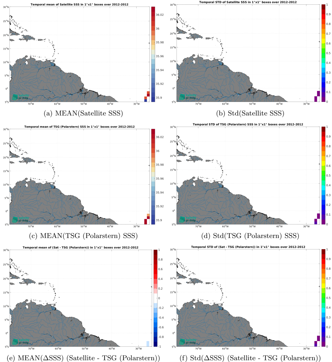
Figure 7: Temporal mean (left) and Std (right) of SSS from Aquarius SSS L3 OR v5 - Monthly - Rain mask (NASA-GSFC) (top), TSG (Polarstern) (middle), and of \Delta SSS (Satellite - TSG (Polarstern)). Only match-up pairs are used to generate these maps.
