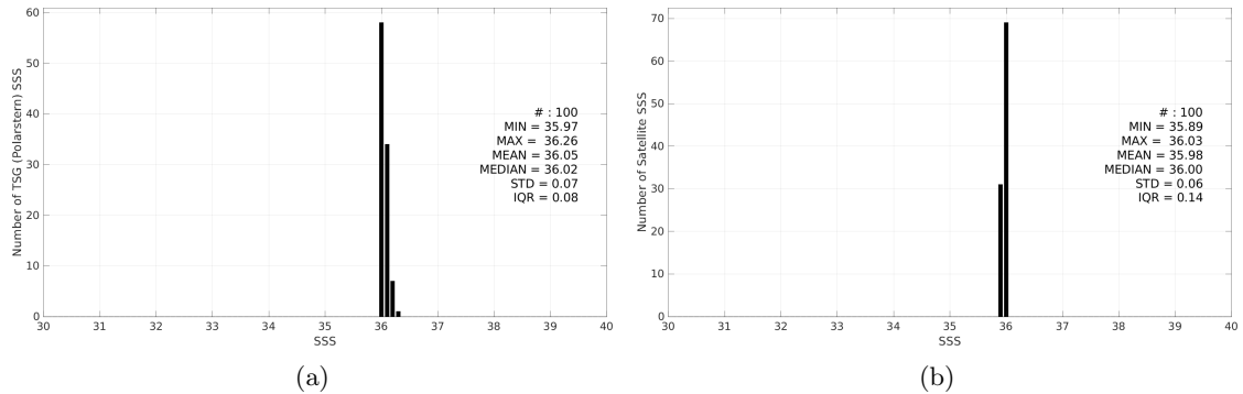
Figure 3: Histograms of SSS from TSG (Polarstern) (a) and Aquarius SSS L3 OR v5 - Monthly - Rain mask (NASA-GSFC) (b) considering all match-up pairs per bins of 0.1 over the Amazon and Orinoco river plumes Pi-MEP region and for the full satellite product period.
